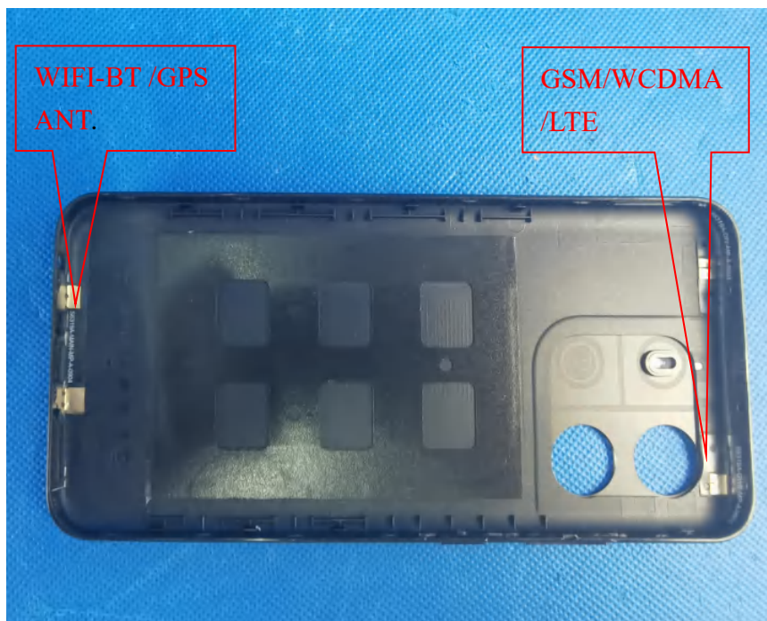
Main ANT
