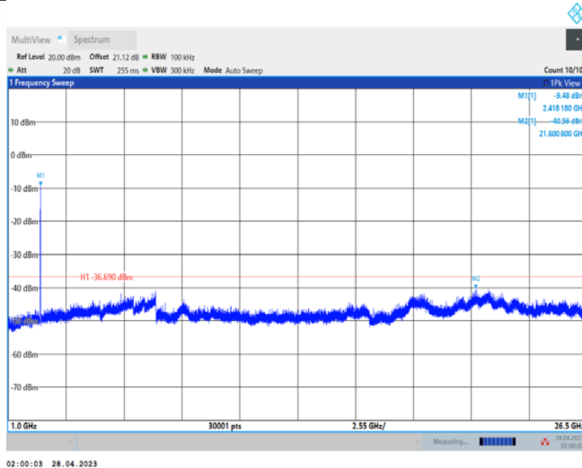
11N20SISO_Ant1_2417_0~Reference
