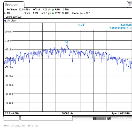
BLE_1M-Ant1-2440-PASS
