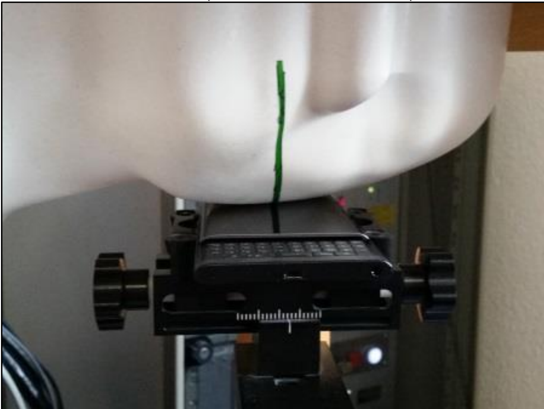
Photo 17: Test position left hand touched slider open
