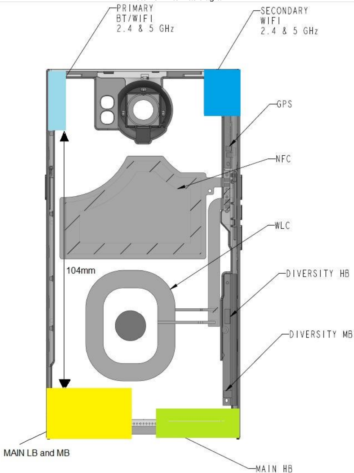
Photo 45: Antennas diagram
