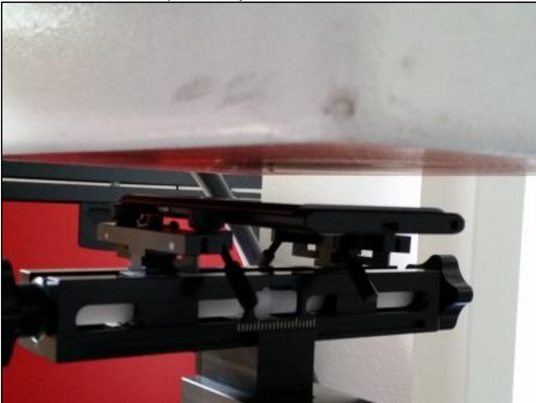
Photo 39: Test position body worn front side with 15 mm distance
