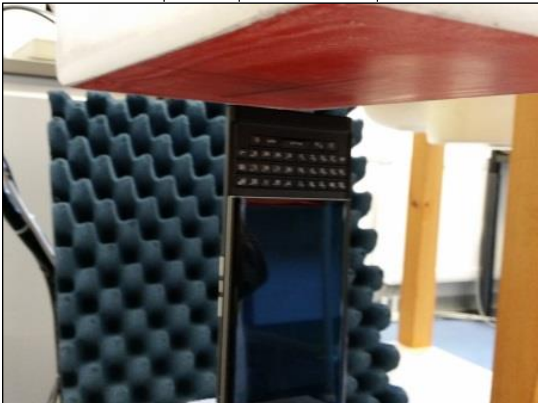
Photo 38: Test position hotspot bottom side slider open with 10 mm
