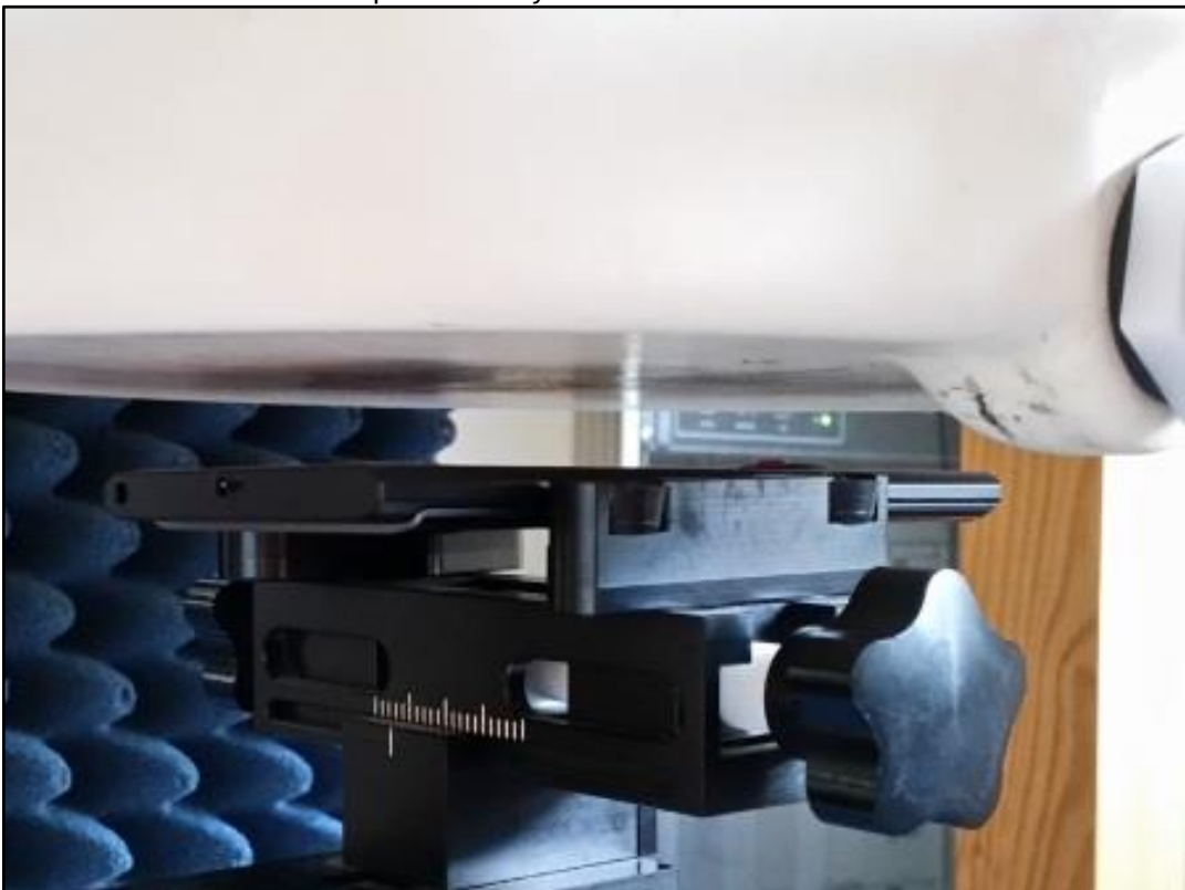
Photo 42: Test position body worn rear side with 15 mm distance
