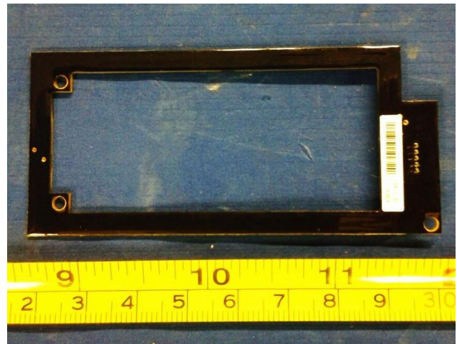
High Frequency Long Antenna Bottom View
