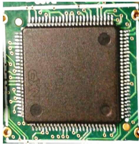
Radio Board Without Shielding
