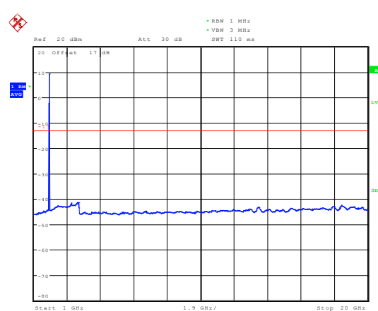
LTE Band 25 1.4MHz CH-Middle 1GHz~20GHz
