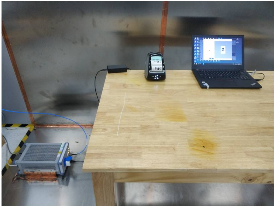
Photograph 3: Set-up photo for Conducted Emissions on AC Mains
