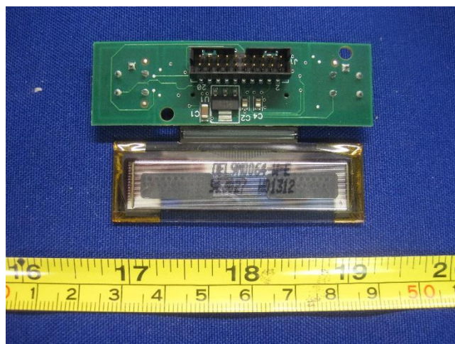
PCBA8 – Bottom View
