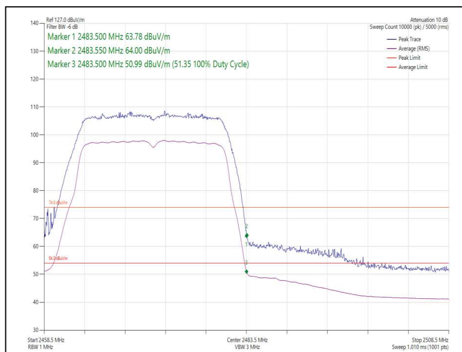
Figure 12 - 802.11n HT20, Core 1 - 2472 MHz, Band Edge Frequency 2483.5 MHz
