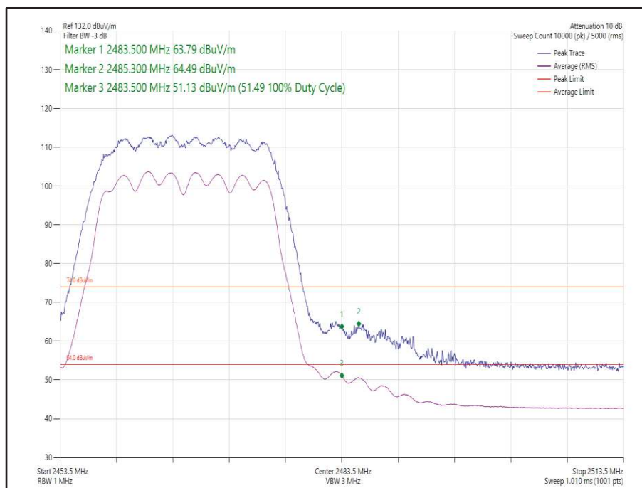
Figure 22 - 802.11n HT20, Core 0-1 - 2467 MHz, Band Edge Frequency 2483.5 MHz
