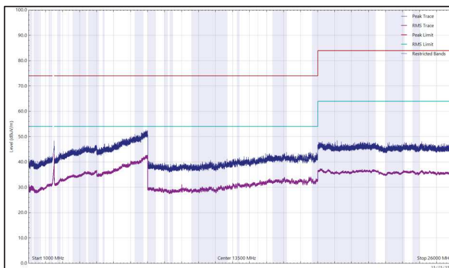
Figure 62 - 2472 MHz (CH13), 802.11b, Core 0, 1 GHz to 26 GHz, Horizontal
