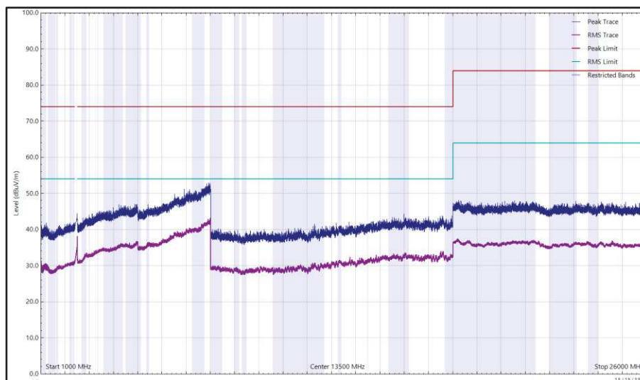
Figure 63 - 2472 MHz (CH13), 802.11b, Core 0, 1 GHz to 26 GHz, Vertical
