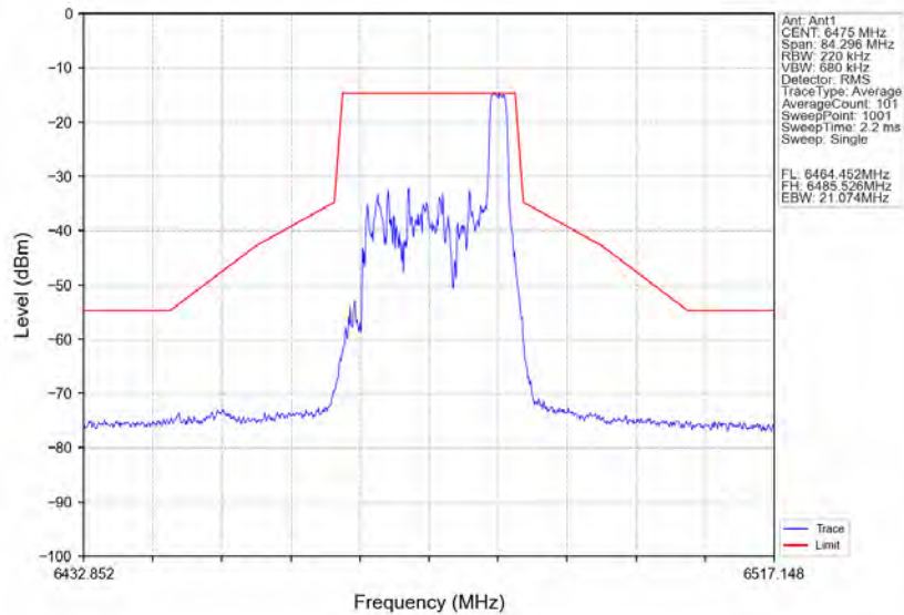
802.11ax(HE20)_MCH_6475MHz_RU26_Right_Ant1_NTNV
