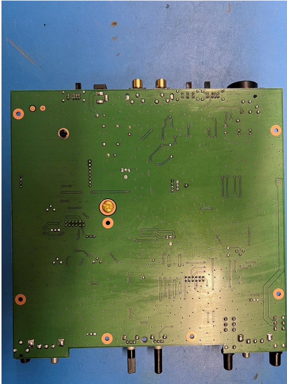
Photograph 2 – Bottom View of the PCBA
