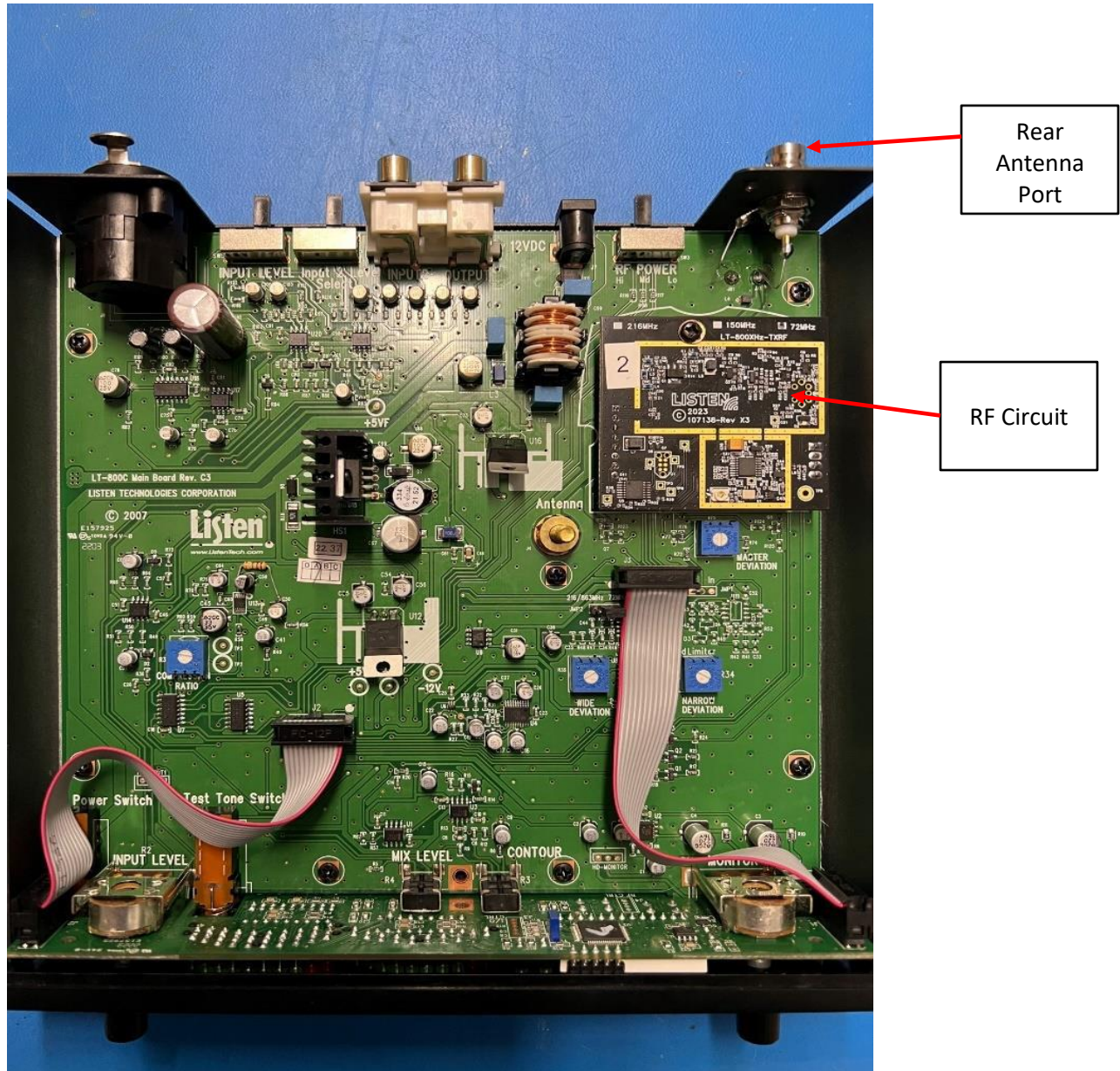
Photograph 1 – Top View of PCB as placed in the Housing
