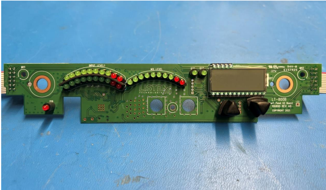
Photograph 5 – Front Panel PCB Front Side
