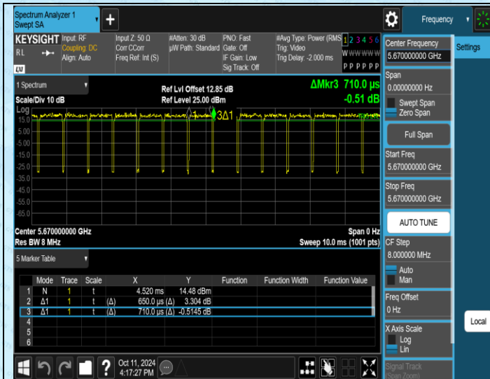
NTNV-11AC40SISO-Ant1-5670
