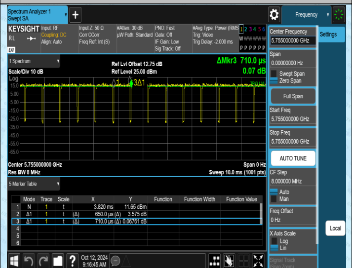
NTNV-11AC40SISO-Ant2-5755
