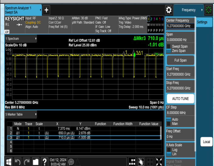
NTNV-11AC40SISO-Ant2-5270
