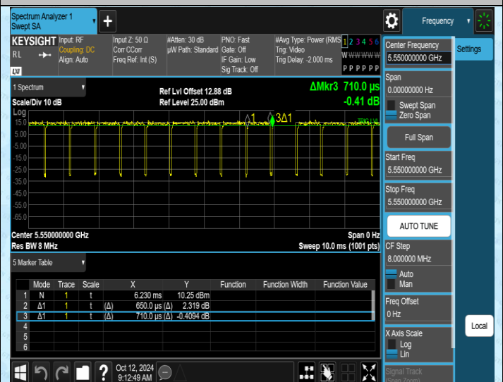
NTNV-11AC40SISO-Ant2-5550
