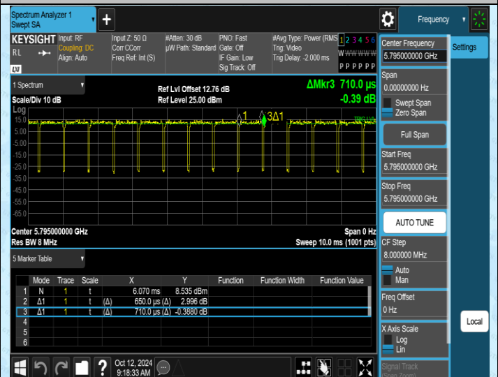
NTNV-11AC40SISO-Ant2-5795
