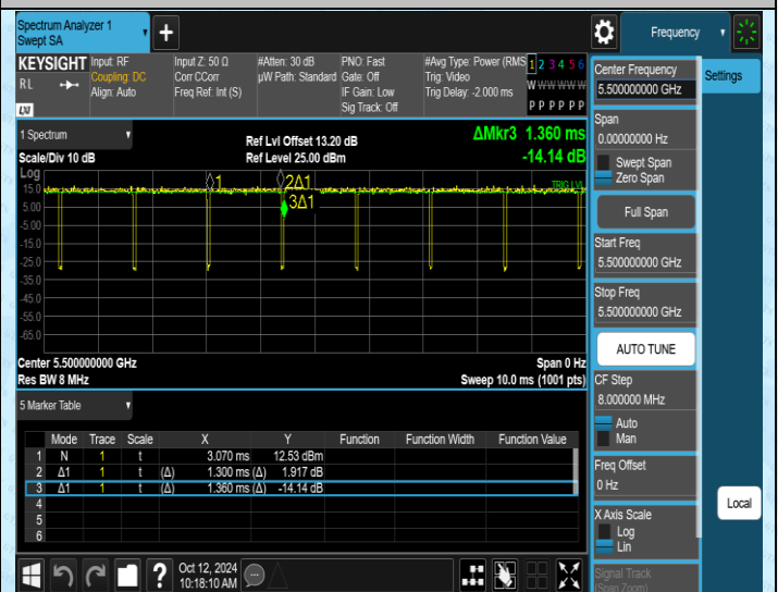
NTNV-11N20MIMO-Ant2-5500
