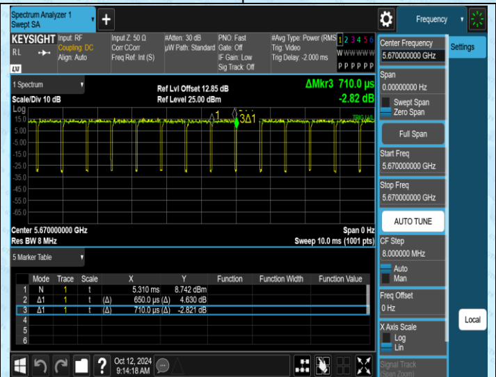
NTNV-11AC40SISO-Ant2-5670
