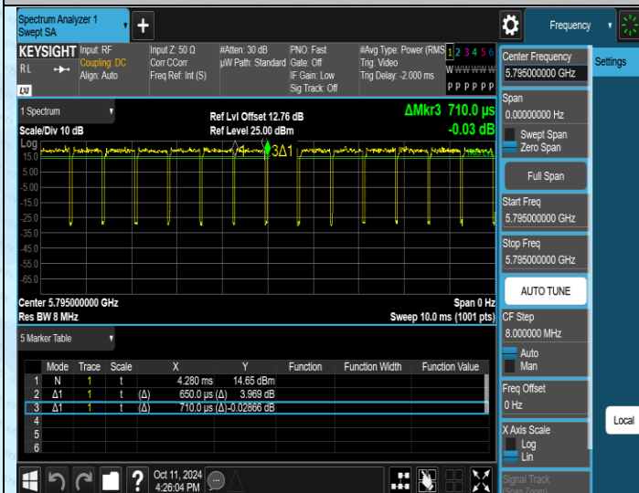
NTNV-11AC40SISO-Ant1-5795
