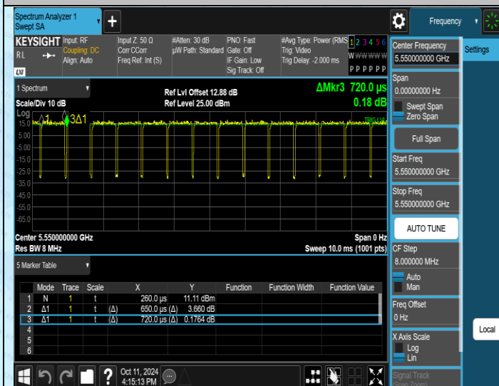
NTNV-11AC40SISO-Ant1-5550
