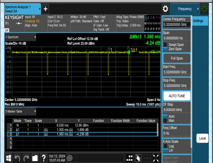
NTNV-11N20MIMO-Ant2-5320
