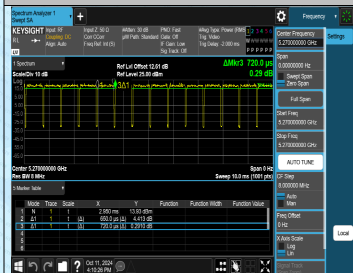
NTNV-11AC40SISO-Ant1-5270
