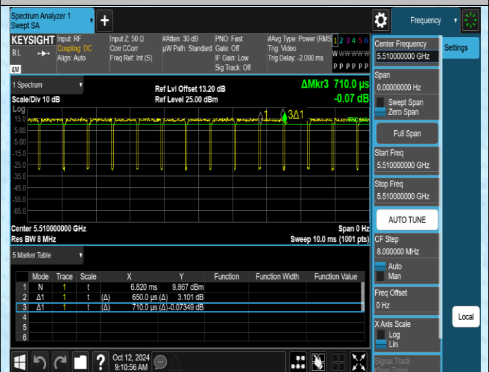
NTNV-11AC40SISO-Ant2-5510
