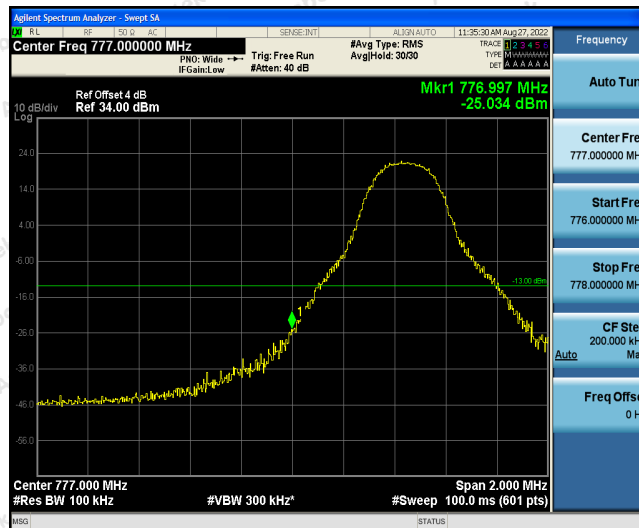
Band13-5MHz-QPSK-23205-1RB#24
