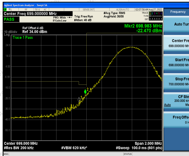
Band12-10MHz-16QAM-23060-1RB#49
