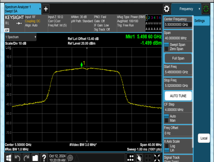
11N20MIMO-Ant2-5500-PASS
