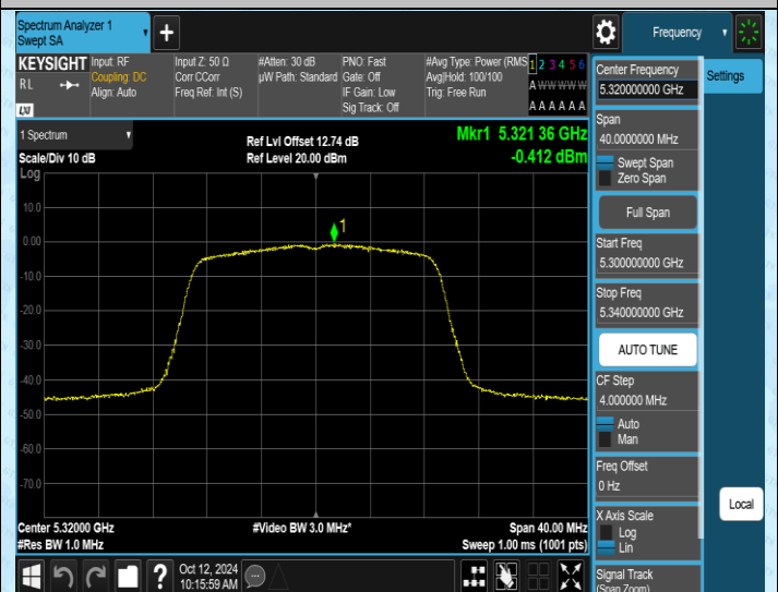
11N20MIMO-Ant2-5320-PASS
