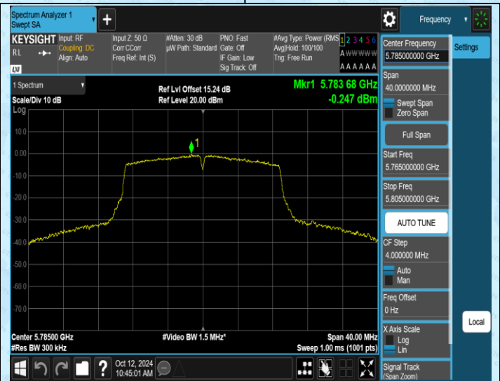
11N20MIMO-Ant2-5785-PASS
