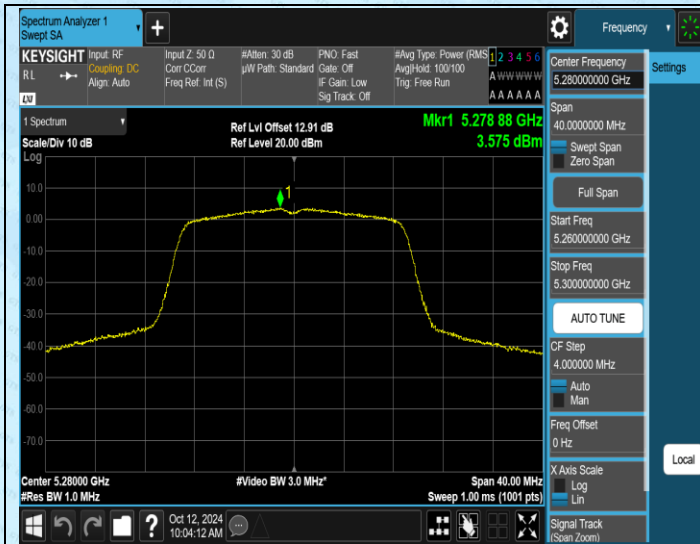
11N20MIMO-Ant1-5280-PASS
