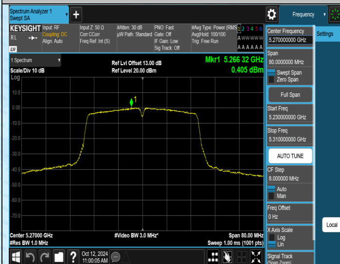
11N40MIMO-Ant1-5270-PASS
