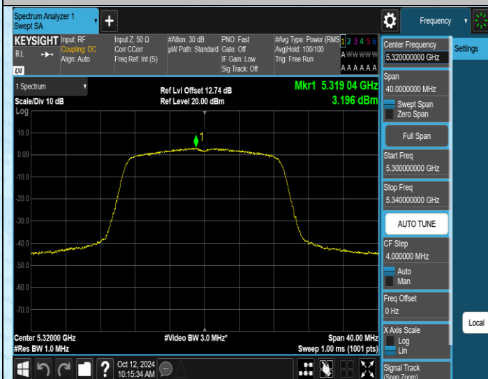
11N20MIMO-Ant1-5320-PASS
