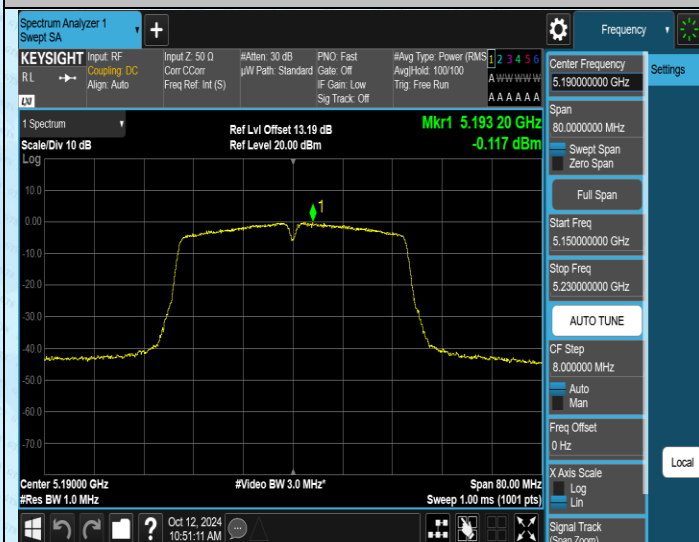
11N40MIMO-Ant1-5190-PASS
