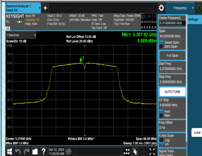
11N40MIMO-Ant1-5310-PASS
