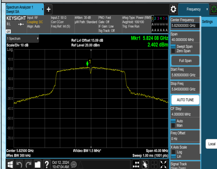
11N20MIMO-Ant1-5825-PASS
