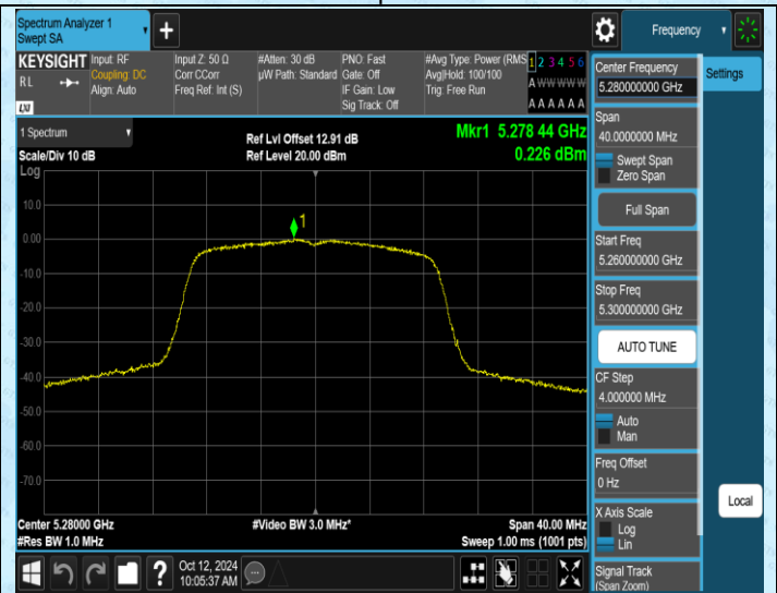
11N20MIMO-Ant2-5280-PASS
