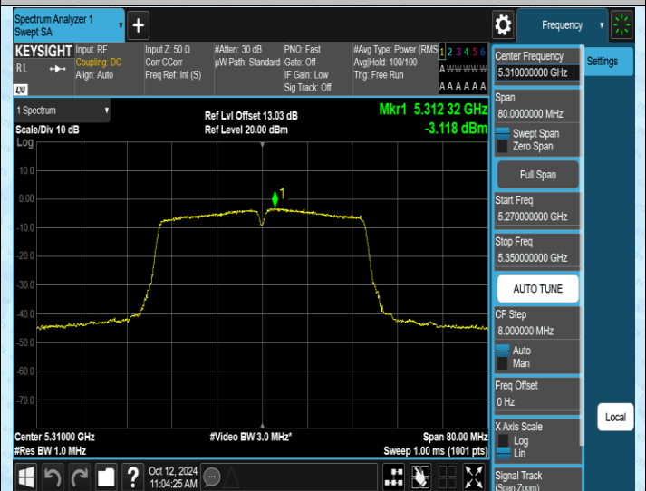
11N40MIMO-Ant2-5310-PASS
