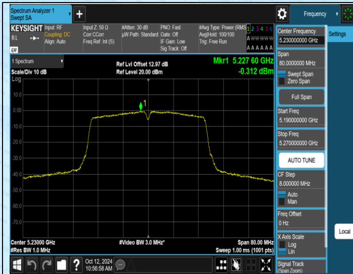
11N40MIMO-Ant1-5230-PASS
