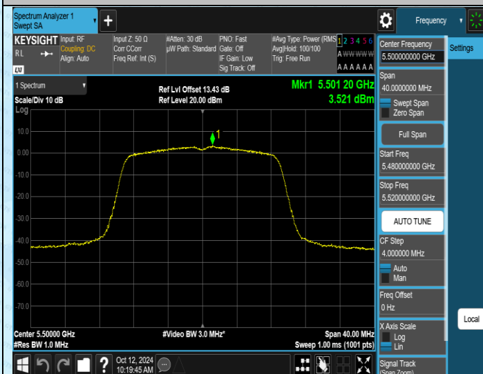
11N20MIMO-Ant1-5500-PASS
