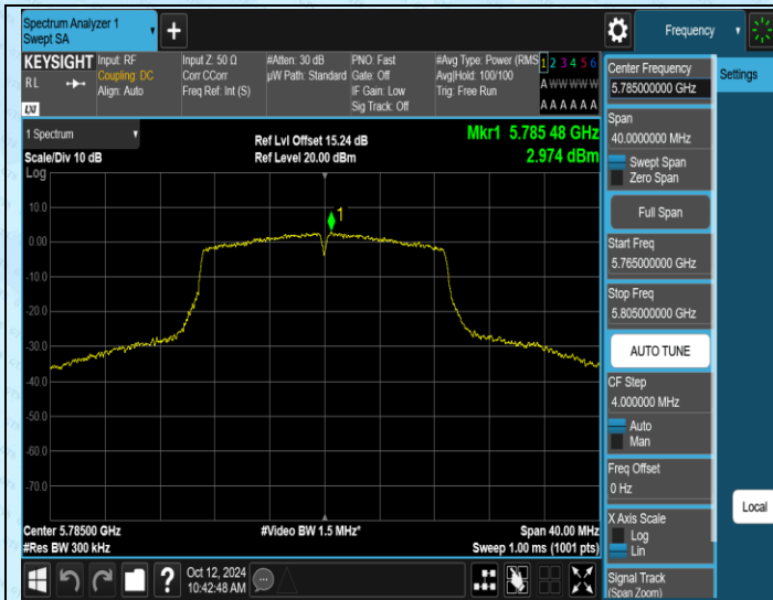
11N20MIMO-Ant1-5785-PASS
