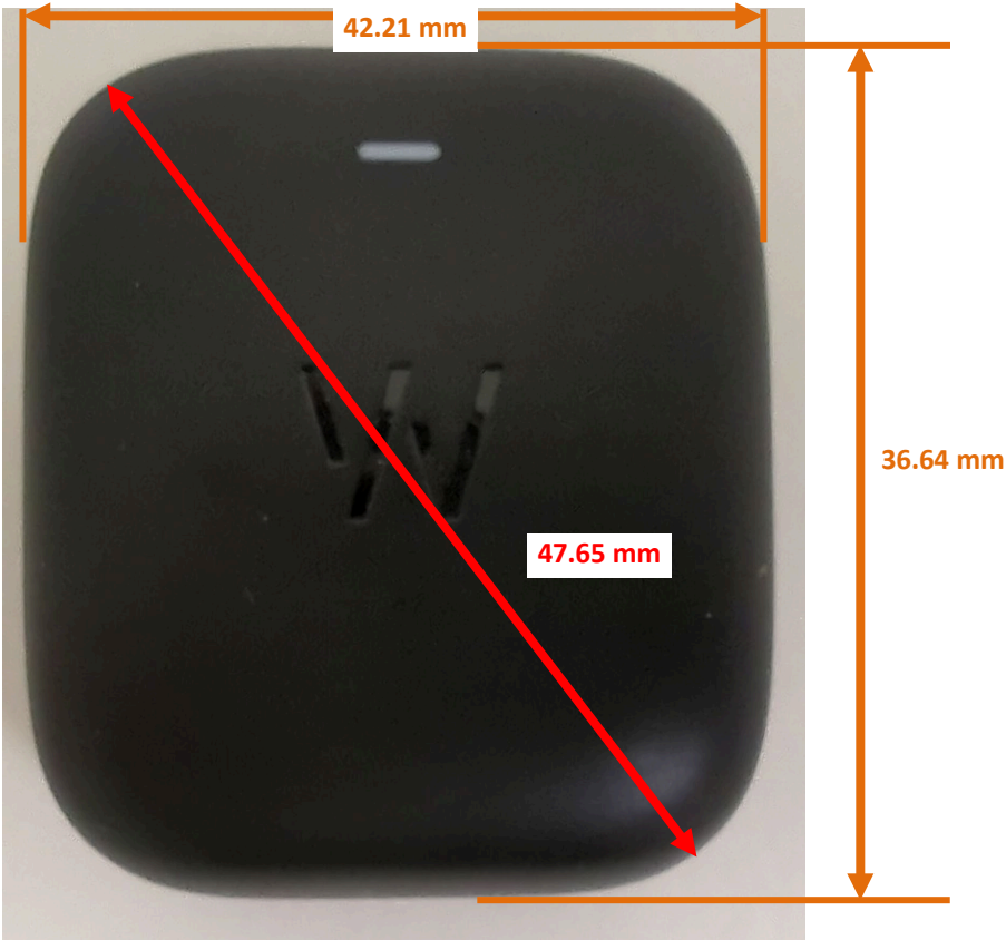
Photograph 1: Overall Dimensions
