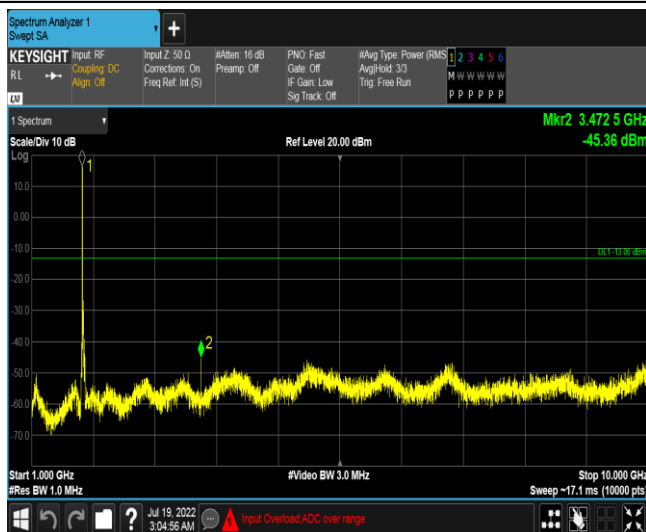
Band66-20MHz-16QAM-132322-1RB#0-Range5:1000~10000MHz
