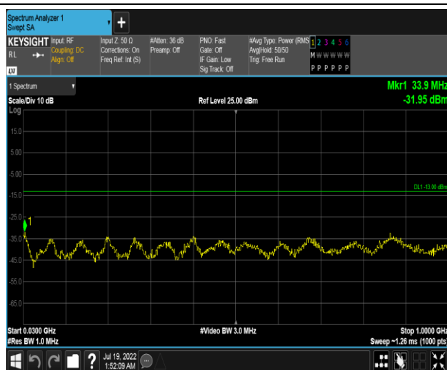
Band66-15MHz-16QAM-132597-1RB#0-Range4:30~1000MHz
