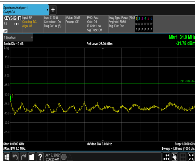
Band66-20MHz-16QAM-132572-1RB#0-Range4:30~1000MHz
