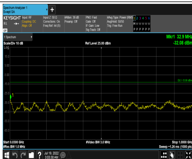
Band66-20MHz-QPSK-132322-1RB#0-Range1:30~1000MHz
