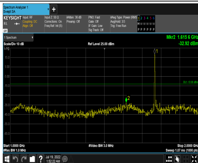
Band66-15MHz-16QAM-132597-1RB#0-Range2:1000~2000MHz
