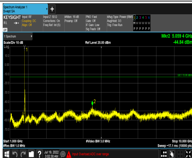
Band66-20MHz-16QAM-132072-1RB#0-Range5:1000~10000MHz
