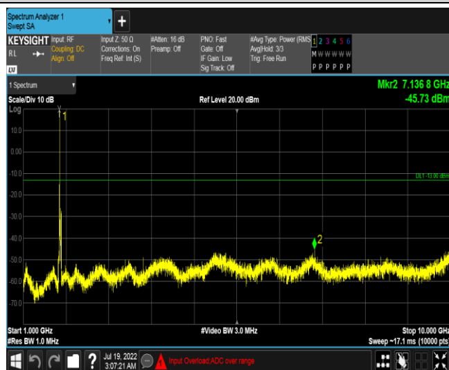
Band66-20MHz-16QAM-132572-1RB#0-Range5:1000~10000MHz
