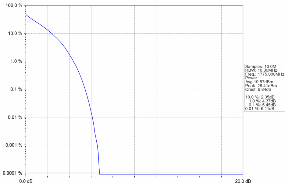
Band66_10MHz_QPSK_HCH_1775MHz_RB_50_0_NTNV
