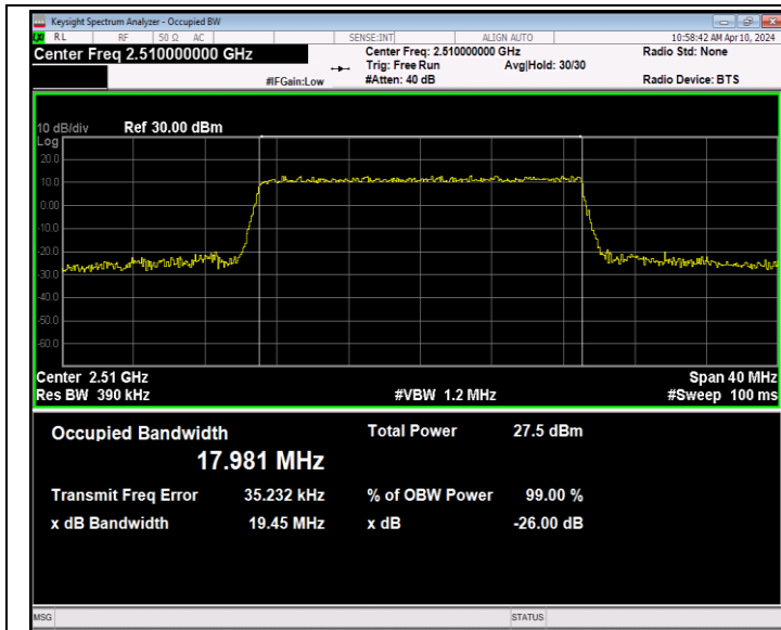
Band7-20MHz-16QAM-20850-100RB#0-PASS
