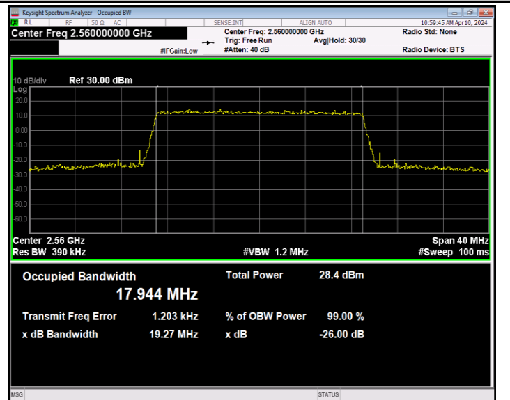
Band7-20MHz-QPSK-21350-100RB#0-PASS
