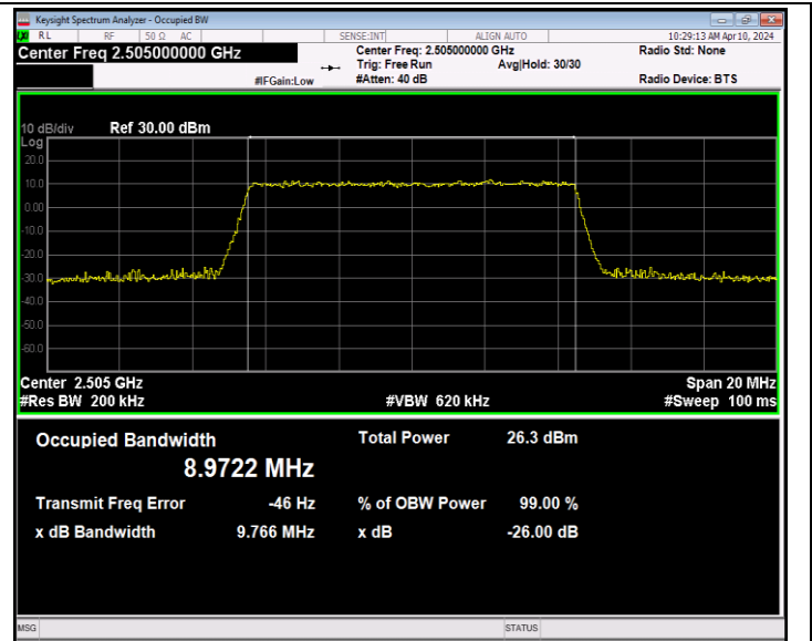
Band7-10MHz-64QAM-20800-50RB#0-PASS
