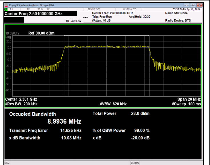
Band41-10MHz-QPSK-39700-50RB#0-PASS
