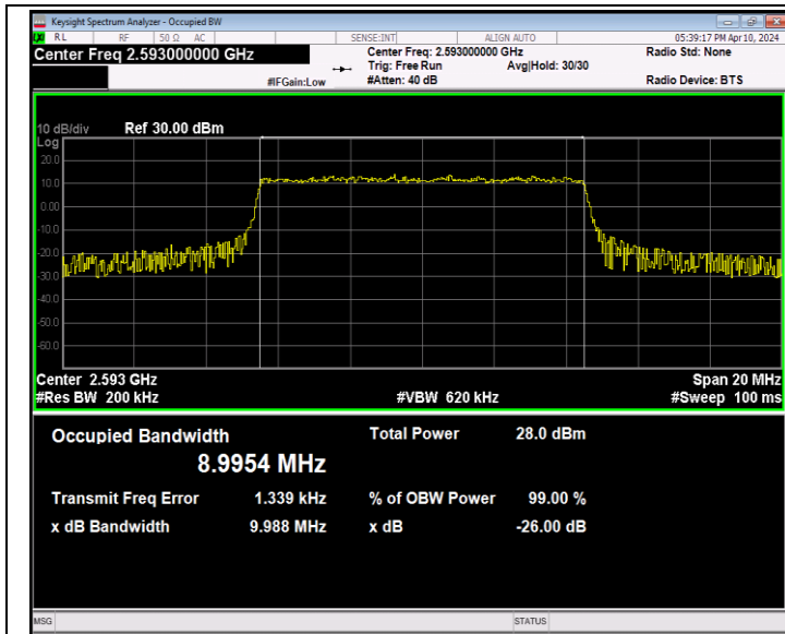
Band41-10MHz-QPSK-40620-50RB#0-PASS
