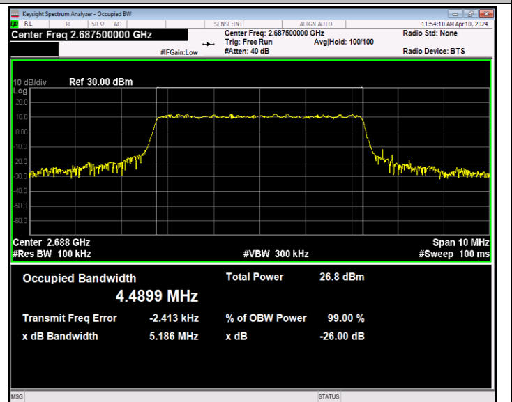
Band41-5MHz-16QAM-41565-25RB#0-PASS
