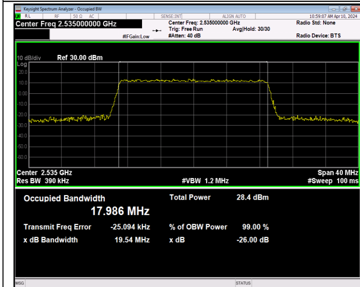
Band7-20MHz-QPSK-21100-100RB#0-PASS
