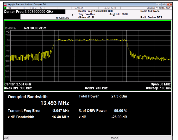
Band41-15MHz-16QAM-39725-75RB#0-PASS
