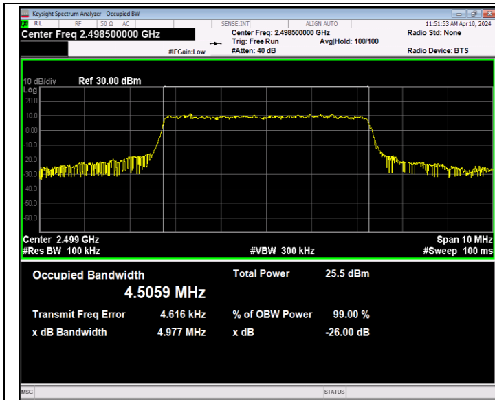
Band41-5MHz-64QAM-39675-25RB#0-PASS
