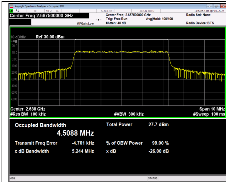
Band41-5MHz-QPSK-41565-25RB#0-PASS
