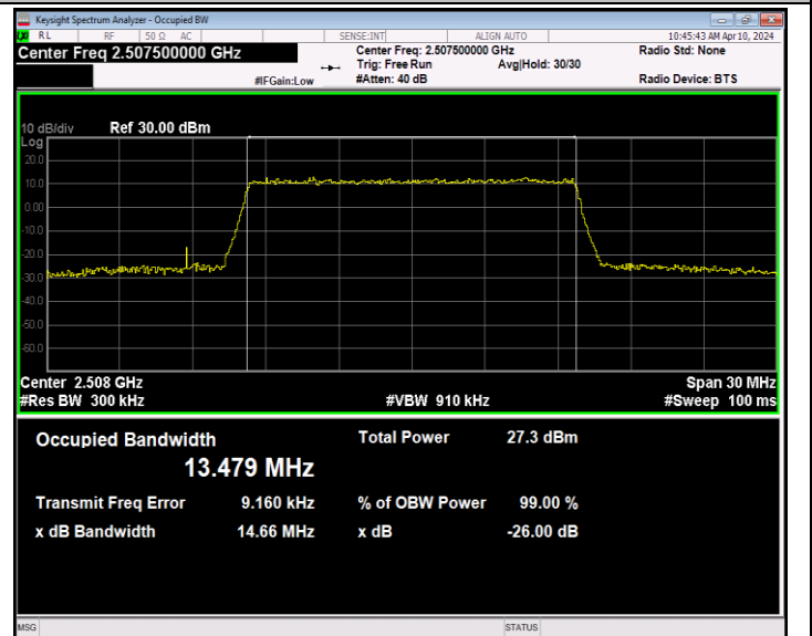
Band7-15MHz-16QAM-20825-75RB#0-PASS
