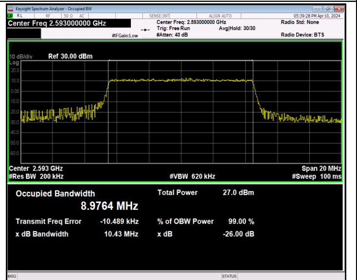
Band41-10MHz-16QAM-40620-50RB#0-PASS
