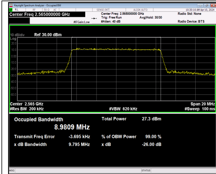
Band7-10MHz-16QAM-21400-50RB#0-PASS
