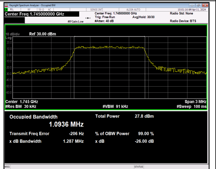
Band66-1.4MHz-QPSK-132322-6RB#0-PASS
