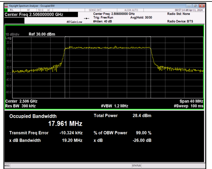
Band41-20MHz-QPSK-39750-100RB#0-PASS
