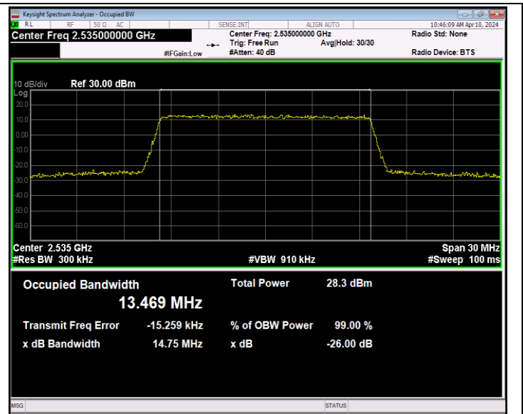
Band7-15MHz-QPSK-21100-75RB#0-PASS
