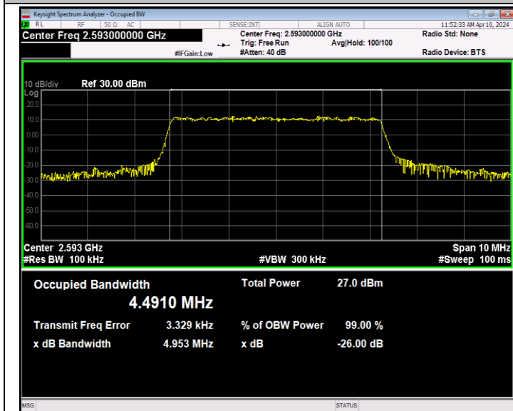
Band41-5MHz-16QAM-40620-25RB#0-PASS
