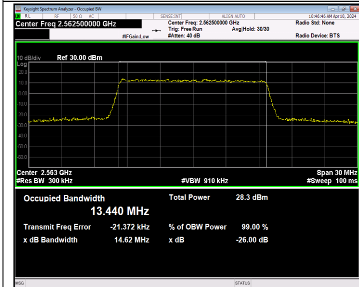
Band7-15MHz-QPSK-21375-75RB#0-PASS
