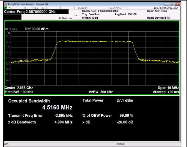
Band7-5MHz-16QAM-21425-25RB#0-PASS
