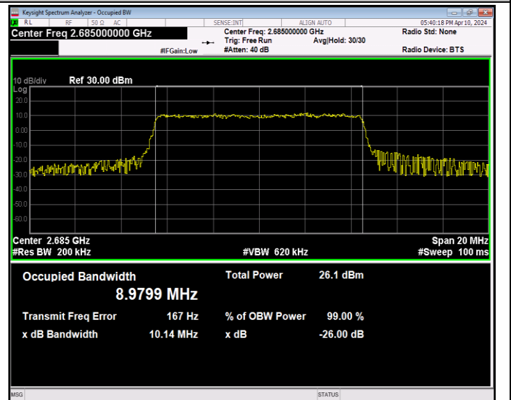
Band41-10MHz-64QAM-41540-50RB#0-PASS
