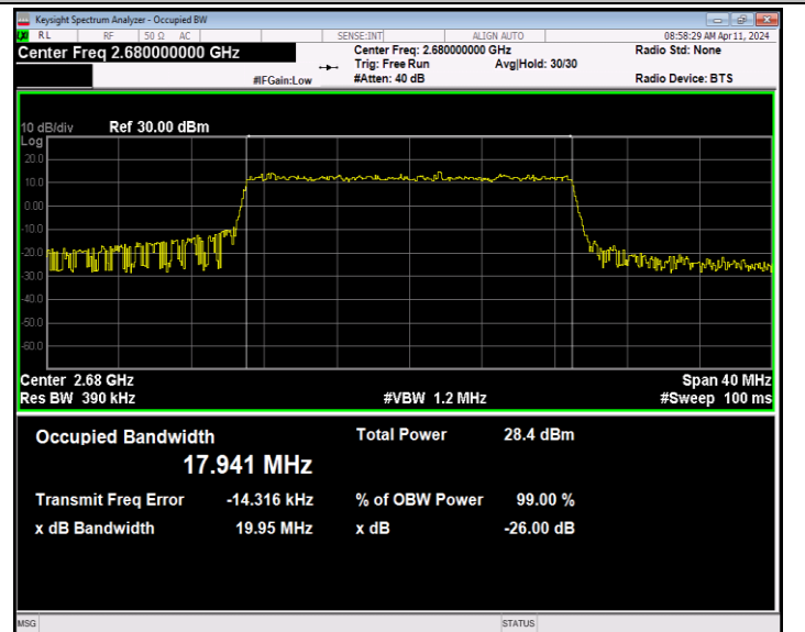
Band41-20MHz-QPSK-41490-100RB#0-PASS
