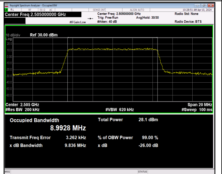
Band7-10MHz-QPSK-20800-50RB#0-PASS
