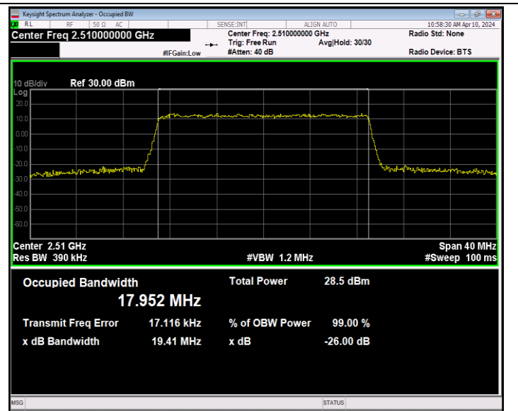
Band7-20MHz-QPSK-20850-100RB#0-PASS
