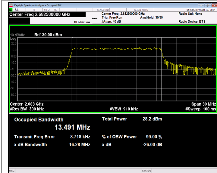
Band41-15MHz-QPSK-41515-75RB#0-PASS
