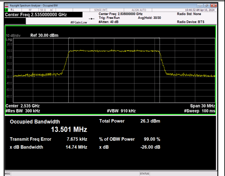
Band7-15MHz-64QAM-21100-75RB#0-PASS
