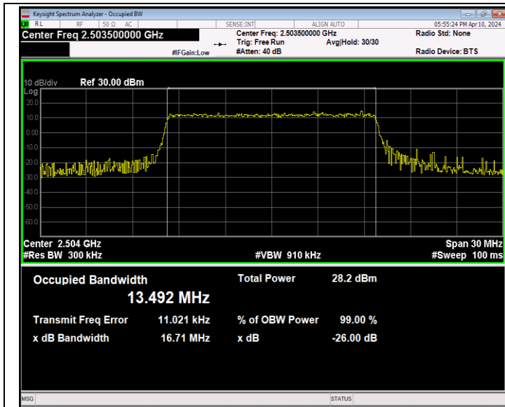
Band41-15MHz-QPSK-39725-75RB#0-PASS
