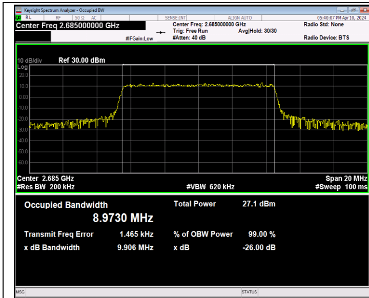
Band41-10MHz-16QAM-41540-50RB#0-PASS
