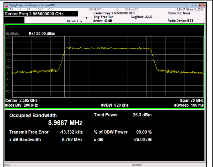
Band7-10MHz-64QAM-21400-50RB#0-PASS
