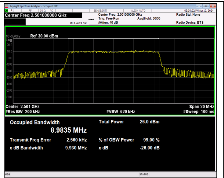
Band41-10MHz-64QAM-39700-50RB#0-PASS
