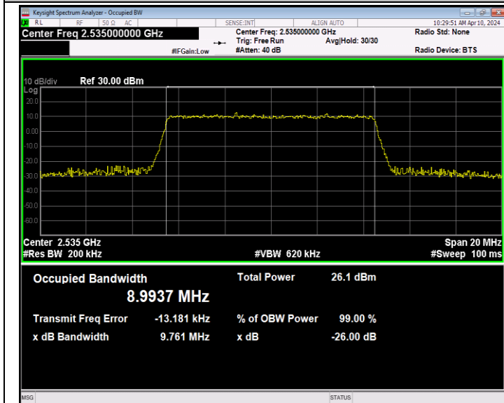
Band7-10MHz-64QAM-21100-50RB#0-PASS
