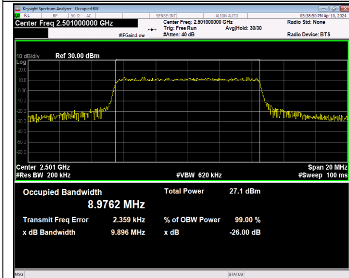
Band41-10MHz-16QAM-39700-50RB#0-PASS
