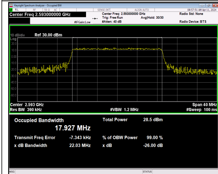
Band41-20MHz-QPSK-40620-100RB#0-PASS
