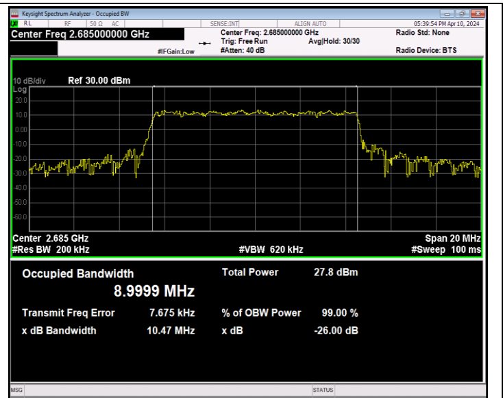
Band41-10MHz-QPSK-41540-50RB#0-PASS
