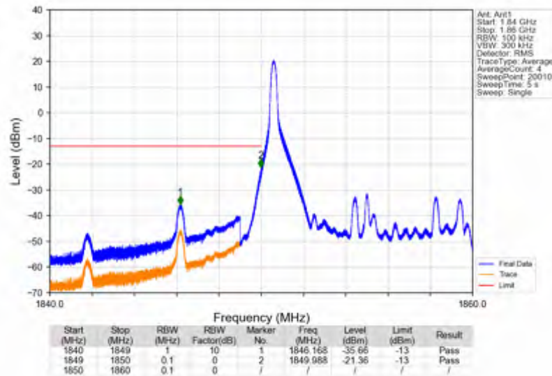
Band25_10MHz_16QAM_LCH_1855MHz_RB_50_0_NTNV
