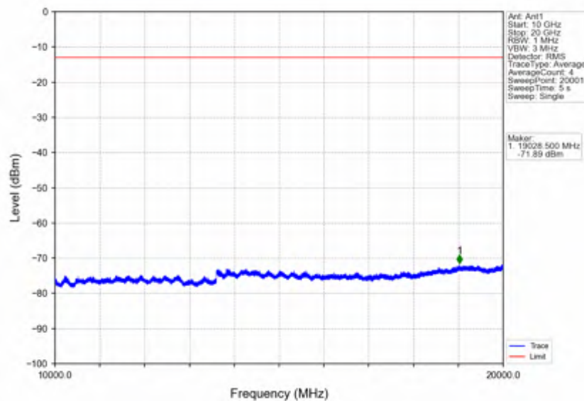
Band25 20MHz 16QAM LCH 1860MHz RB 100 0 NTN
