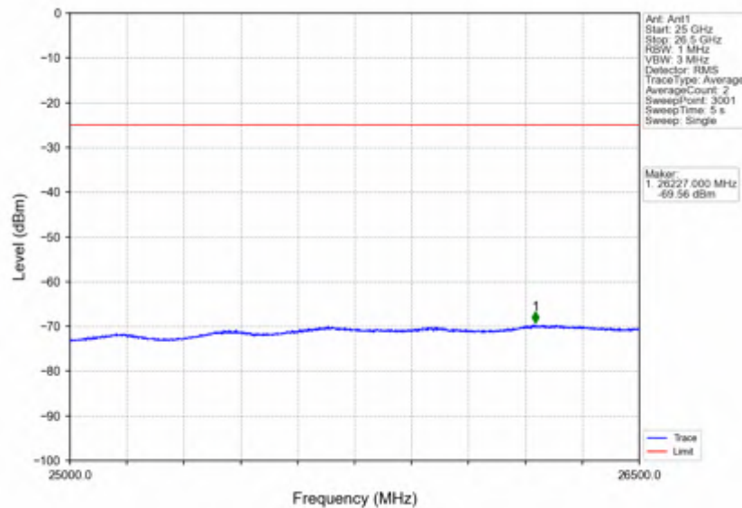
Band7_15MHz_64QAM_LCH_2507.5MHz_RB_1_0_NTNV
