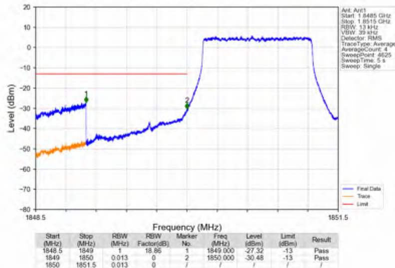
Band25_1.4MHz_QPSK_LCH_1850.7MHz_RB_6_0_NTNV
