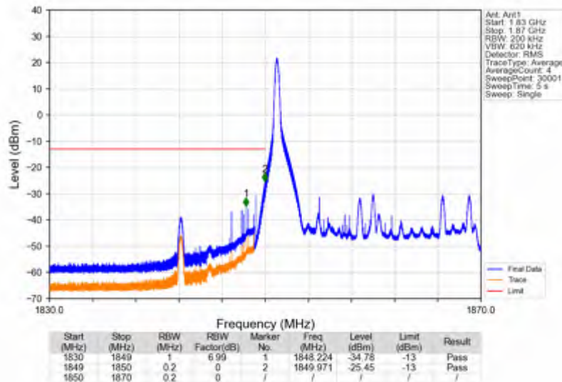
Band25_20MHz_64QAM_LCH_1860MHz_RB_100_0_NTNV
