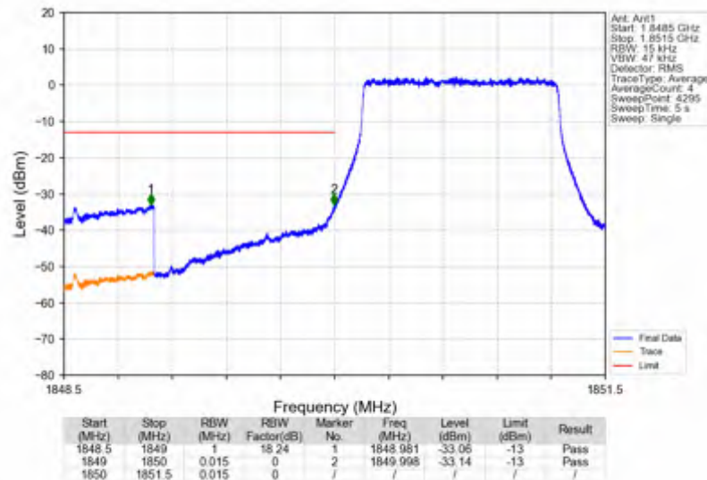
Band25_1.4MHz_256QAM_LCH_1850.7MHz_RB_6_0_NTNV
