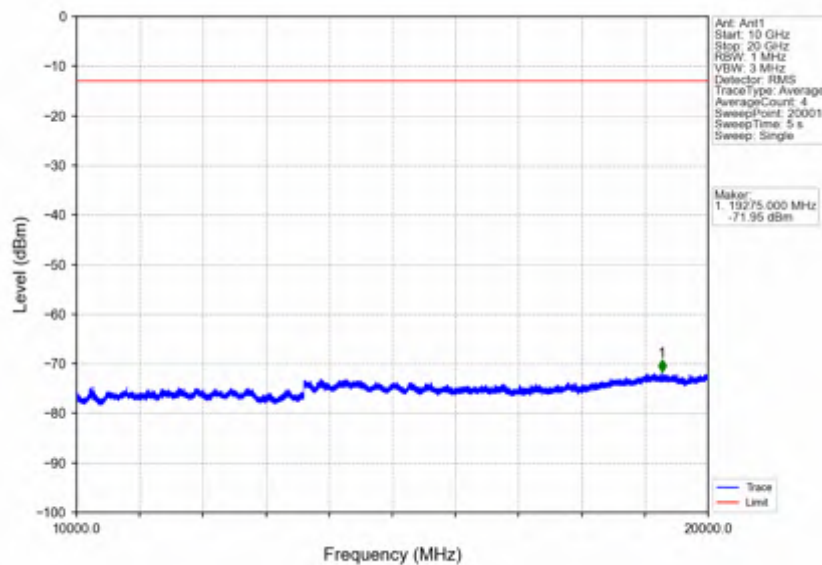
Band25 5MHz QPSK HCH 1912.5MHz RB 1 0 NTNV
