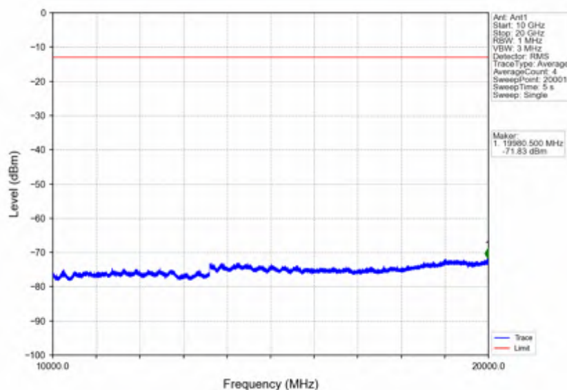
Band25 1.4MHz 16QAM LCH 1850.7MHz RB 6 0 NTNV
