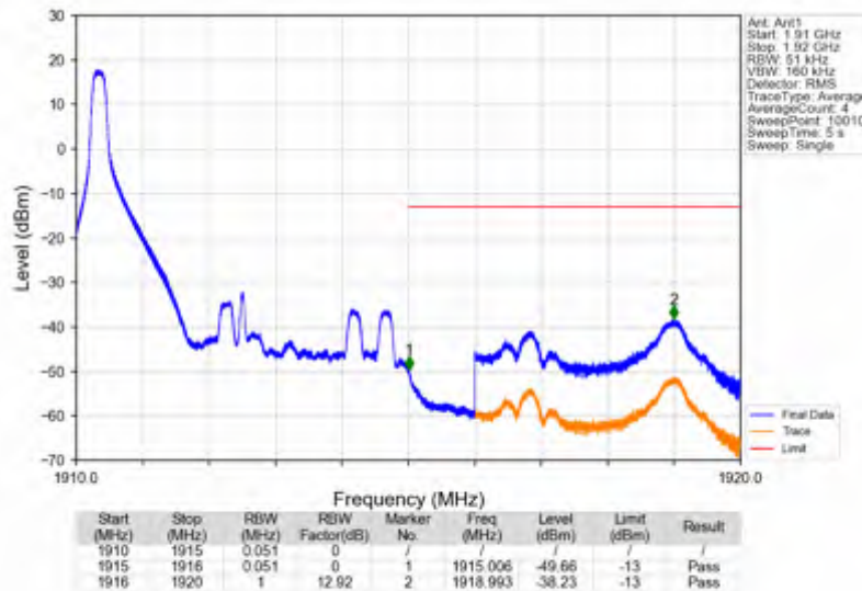
Band25_5MHz_16QAM_HCH_1912.5MHz_RB_1_24_NTNV
