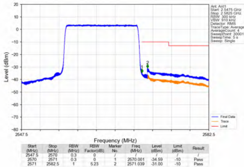
Band7_15MHz_256QAM_HCH_2562.5MHz_RB_75_0_NTNV
