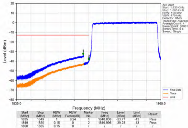
Band25_15MHz_256QAM_LCH_1857.5MHz_RB_75_0_NTNV
