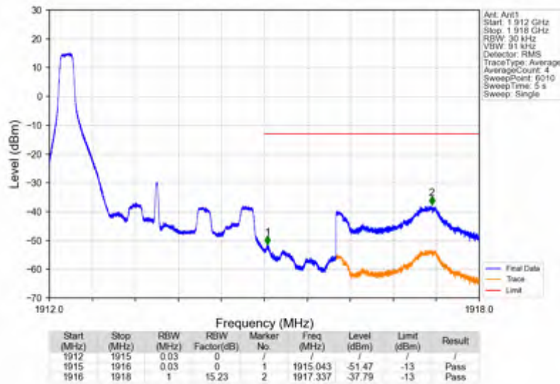
Band25_3MHz_16QAM_HCH_1913.5MHz_RB_1_14_NTNV
