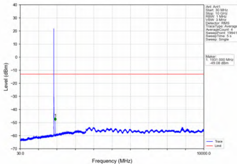
Band25_10MHz_64QAM_LCH_1855MHz_RB_1_0_NTV
