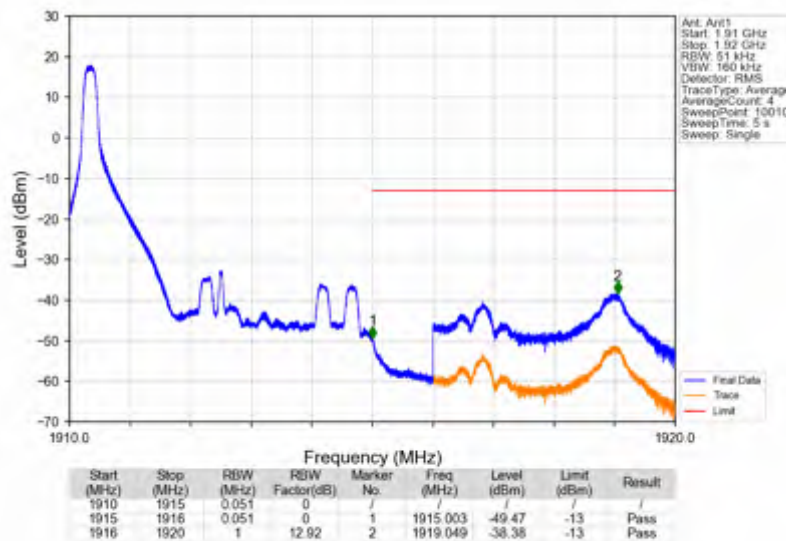
Band25_5MHz_16QAM_HCH_1912.5MHz_RB_25_0_NTNV
