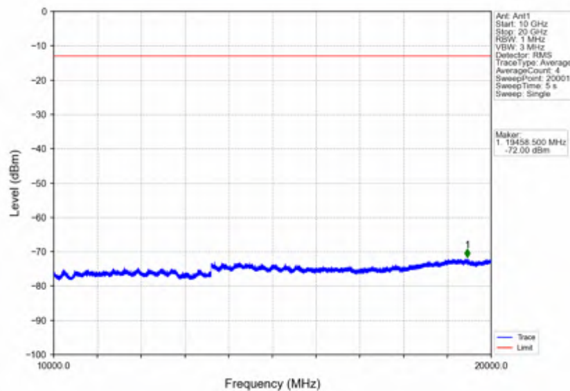
Band25_20MHz_256QAM_LCH_1860MHz_RB_100_0_NTNV
