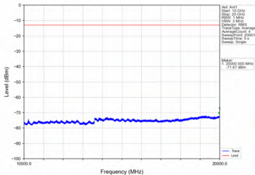
Band25_3MHz_64QAM_HCH_1913.5MHz_RB_1_0_NTNV
