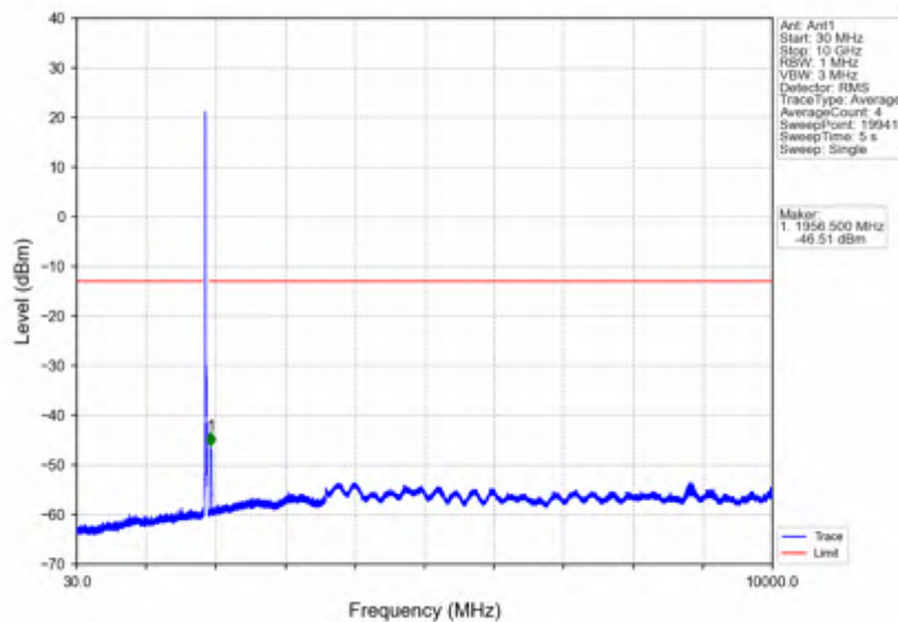
Band25 20MHz 64QAM MCH 1882.5MHz RB 1 0 NTNv
