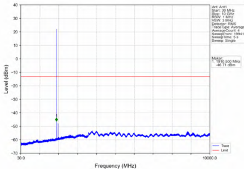
Band25_1.4MHz_64QAM_HCH_1914.3MHz_RB_1_0_NTNV
