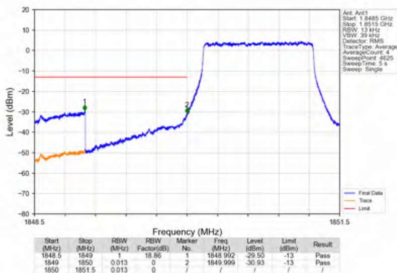
Band25 1.4MHz 16QAM LCH 1850.7MHz RB 6 0 NTNV
