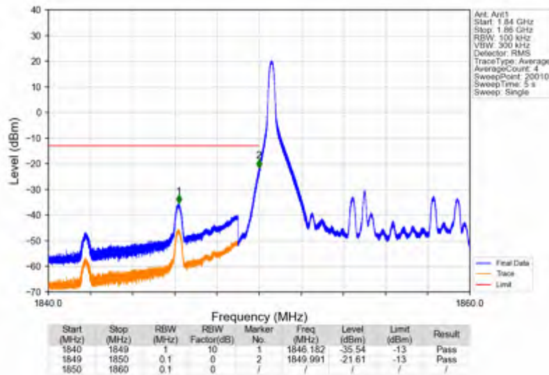
Band25_10MHz_64QAM_LCH_1855MHz_RB_1_0_NTV
