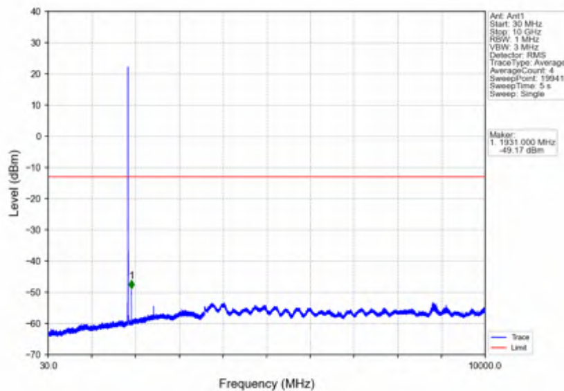
Band25 5MHz 64QAM LCH 1852.5MHz RB 1 0 NTNV
