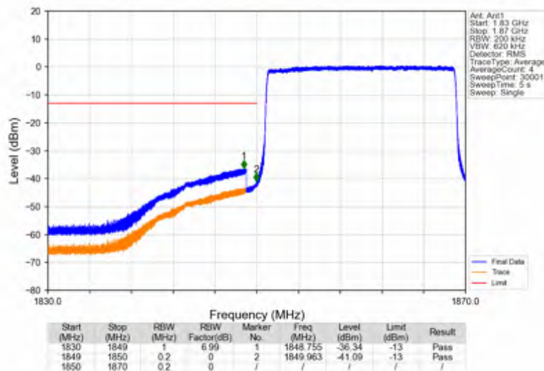
Band25_20MHz_256QAM_LCH_1860MHz_RB_100_0_NTNV
