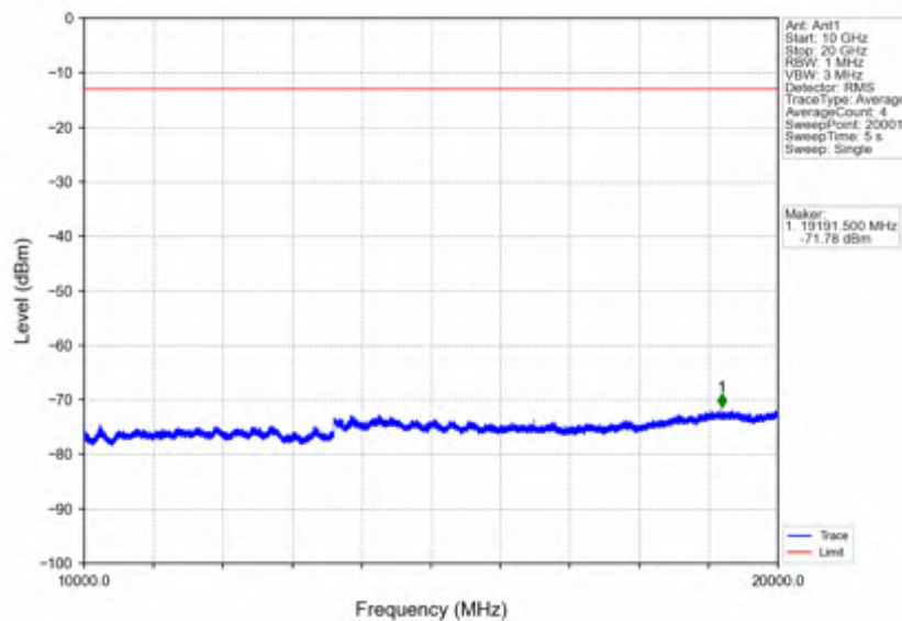
Band25_5MHz_QPSK_MCH_1882.5MHz_RB_1_0_NTNV
