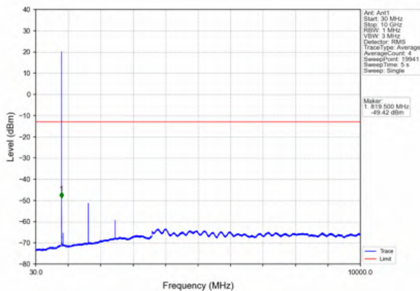
Band26a_1.4MHz_16QAM_HCH_823.3MHz_RB_1_0_NTNV
