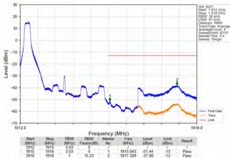
Band25_3MHz_16QAM_HCH_1913.5MHz_RB_15_0_NTNV
