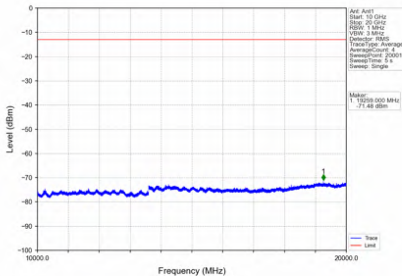
Band25_10MHz_16QAM_HCH_1910MHz_RB_1_0_NTNV
