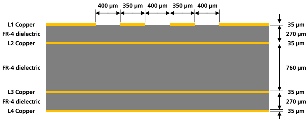
Figure 59: Example of USB line design, with Z_o close to 90 \Omega and Z_{CM} close to 30 \Omega , for the described 4-layer board layup
