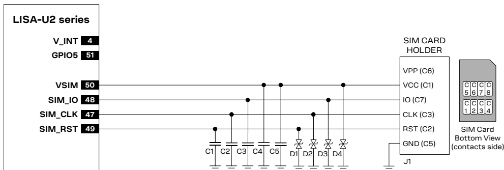
Figure 21: Application circuit for the connection to a single removable SIM card, with SIM detection not implemented
