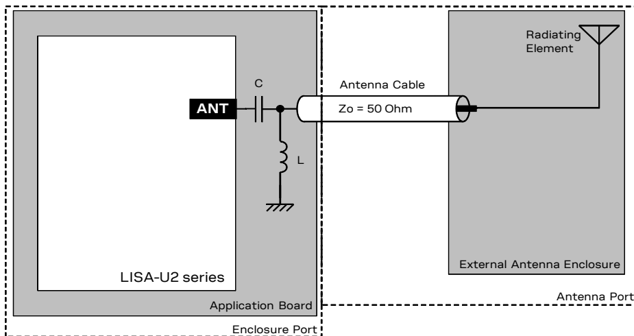
Figure 68: Antenna port ESD immunity protection application circuit for LISA-U2 series modules
