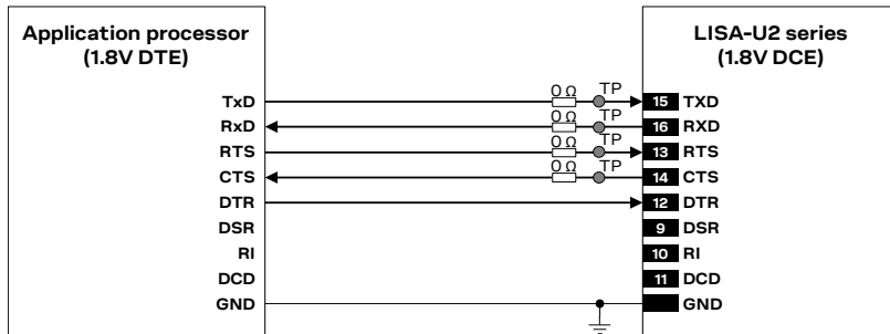
Figure 33: UART interface application circuit with partial V.24 link (6-wire) in the DTE/DCE serial communication (1.8 V DTE)
