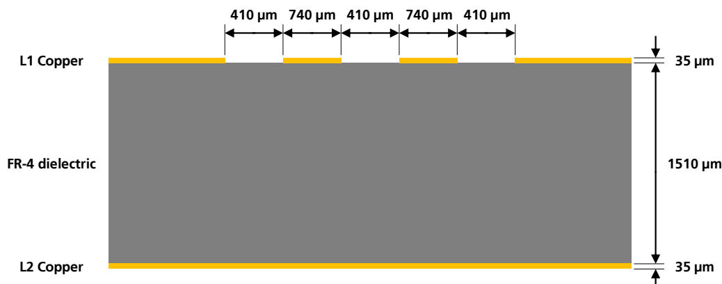
Figure 60: Example of USB line design, with Z_o close to 90 \Omega and Z_{CM} close to 30 \Omega , for the described 2-layer board layup
