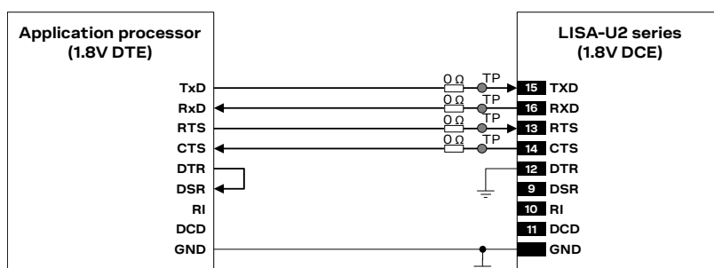
Figure 35: UART interface application circuit with partial V.24 link (5-wire) in the DTE/DCE serial communication (1.8 V DTE)
