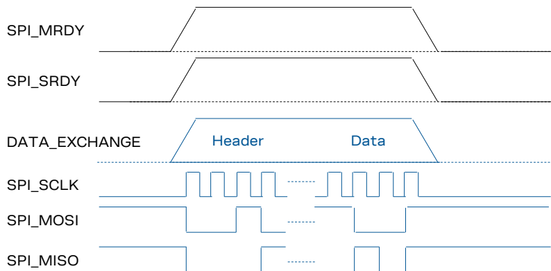
Figure 41: IPC Data Flow: SPI_MRDY and SPI_SRDY line usage combined with the SPI protocol
