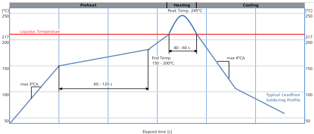
Figure 74: Recommended soldering profile
