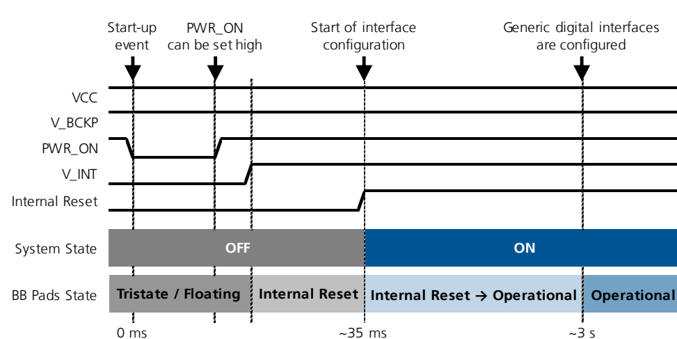
Figure 18: LISA-U2 series power-on sequence description
