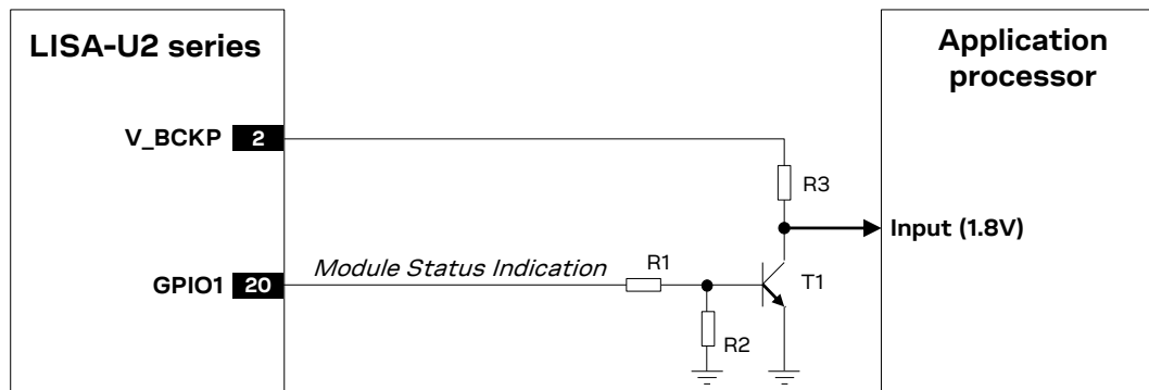
Figure 53: Module status indication application circuit
