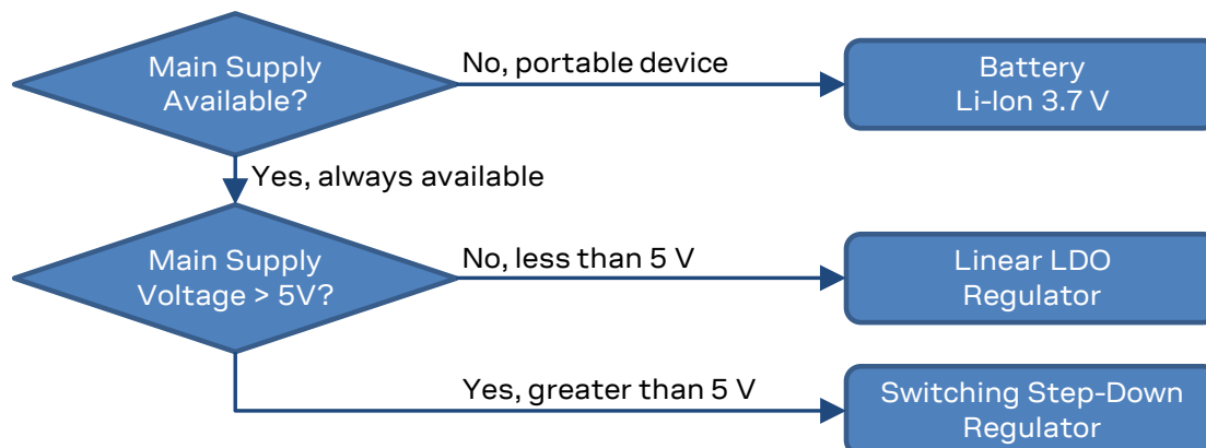
Figure 5: VCC supply concept selection
