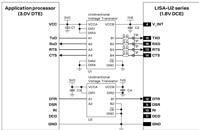
Figure 34: UART interface application circuit with partial V.24 link (6-wire) in DTE/DCE serial communication (3.0 V DTE)
