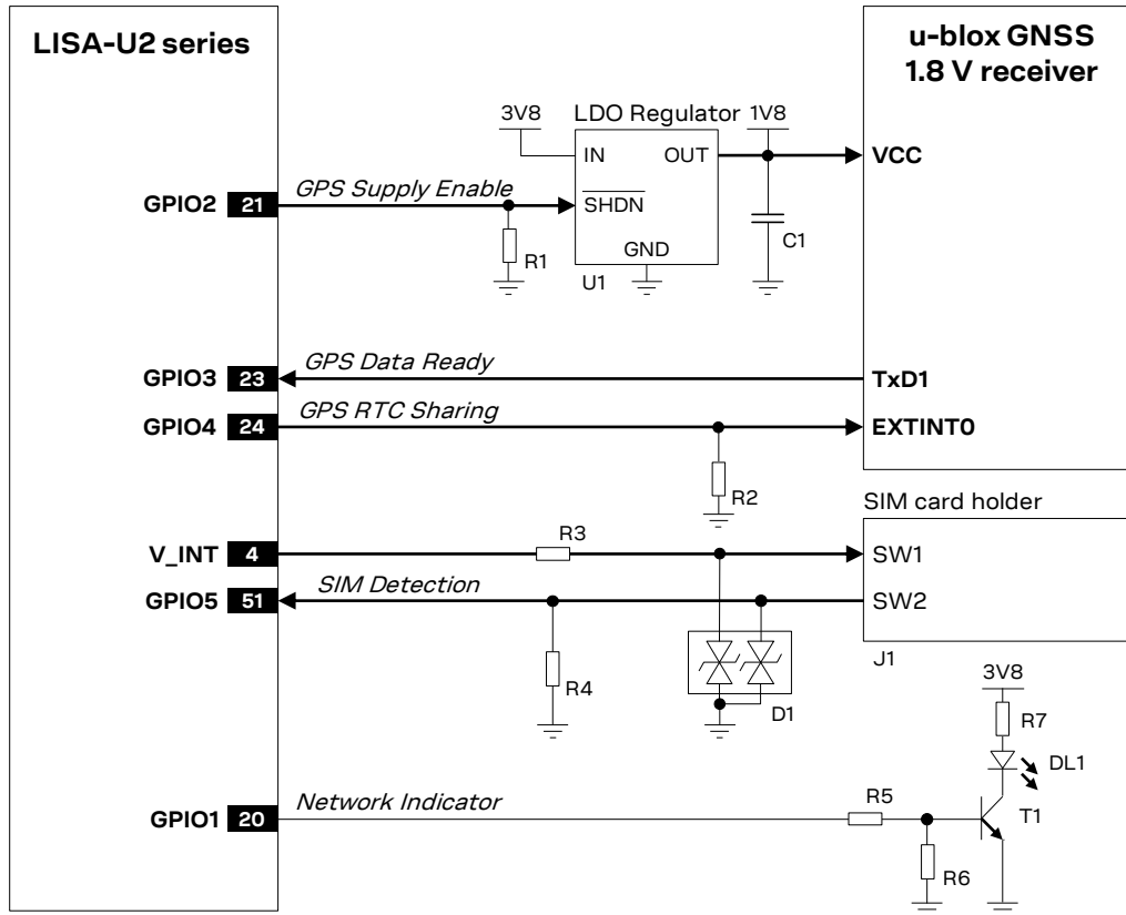
Figure 52: GPIO application circuit
