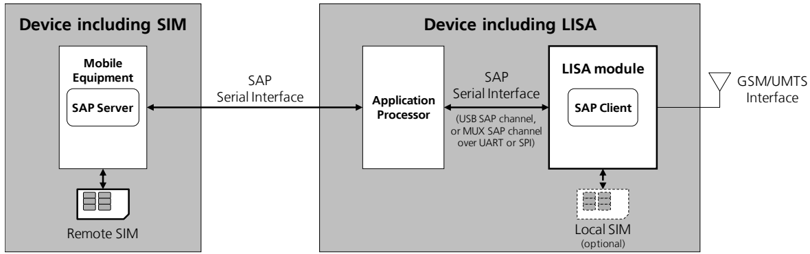
Figure 70: Remote SIM access via completely wired connection
