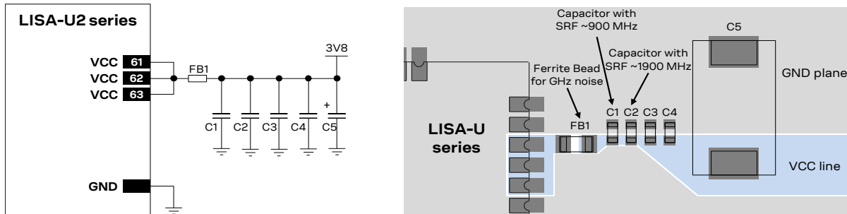
Figure 9: Suggested schematic and layout design for the VCC line; highly recommended when using an integrated antenna
