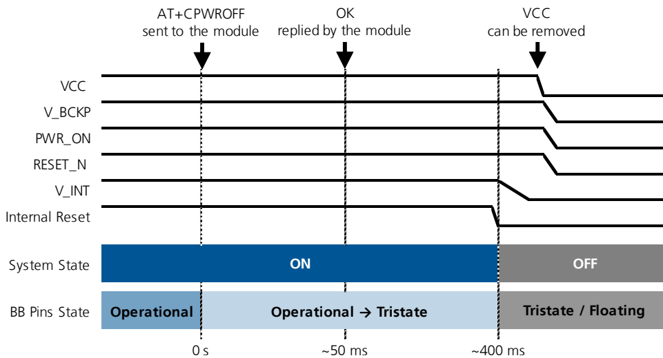
Figure 19: LISA-U2 series Power-off sequence description
