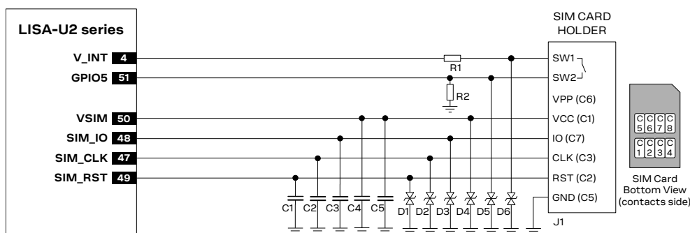
Figure 23: Application circuit for connection to a single removable SIM card, with SIM detection implemented
