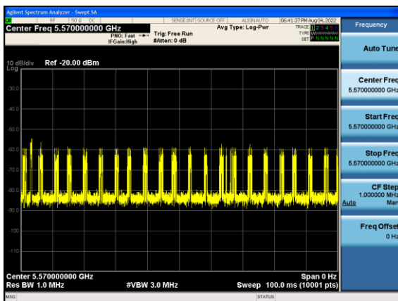
802.11ax-HE160 (5570MHz)
