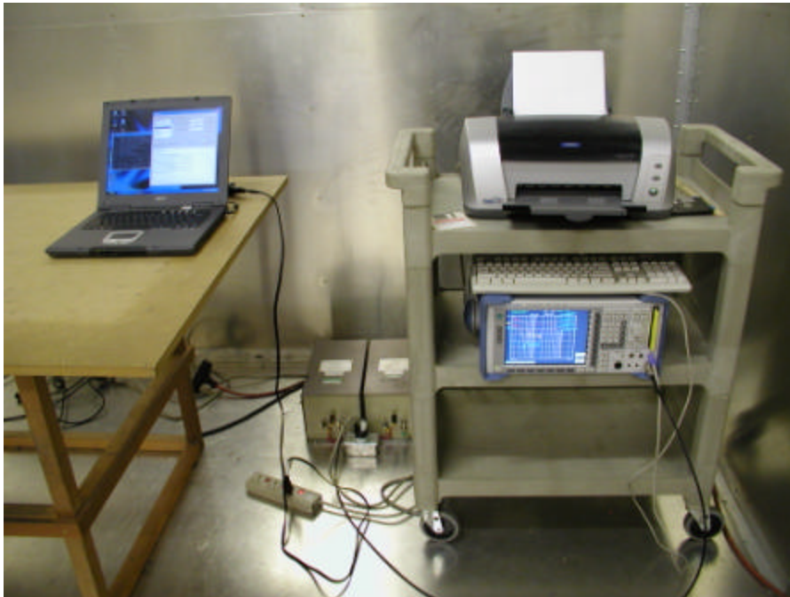
Conducted Emission - Front View, ZG1S Antenna
