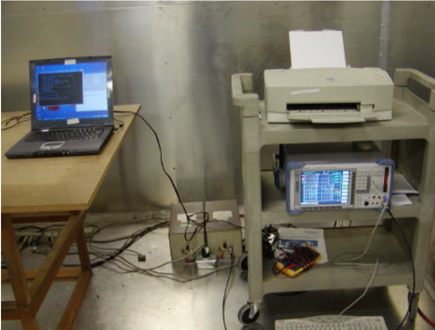
Conducted Emission - Front View, ZIIS Antenna
