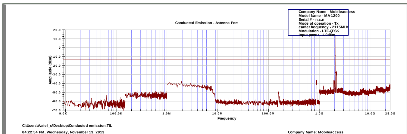
Figure 44.— QPSK (Low)
