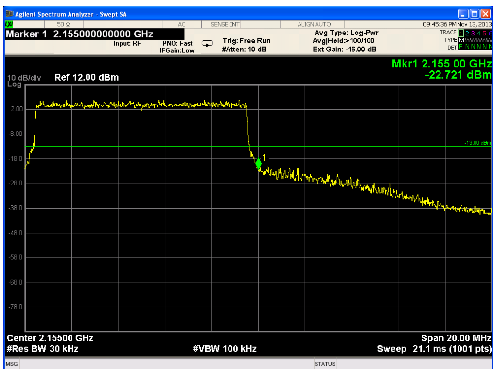
Figure 51.— 64QAM HIGH
