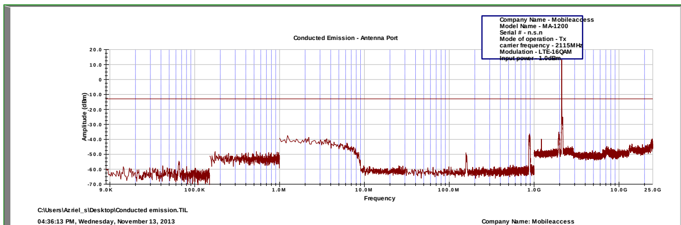
Figure 38.— 16QAM (Low)
