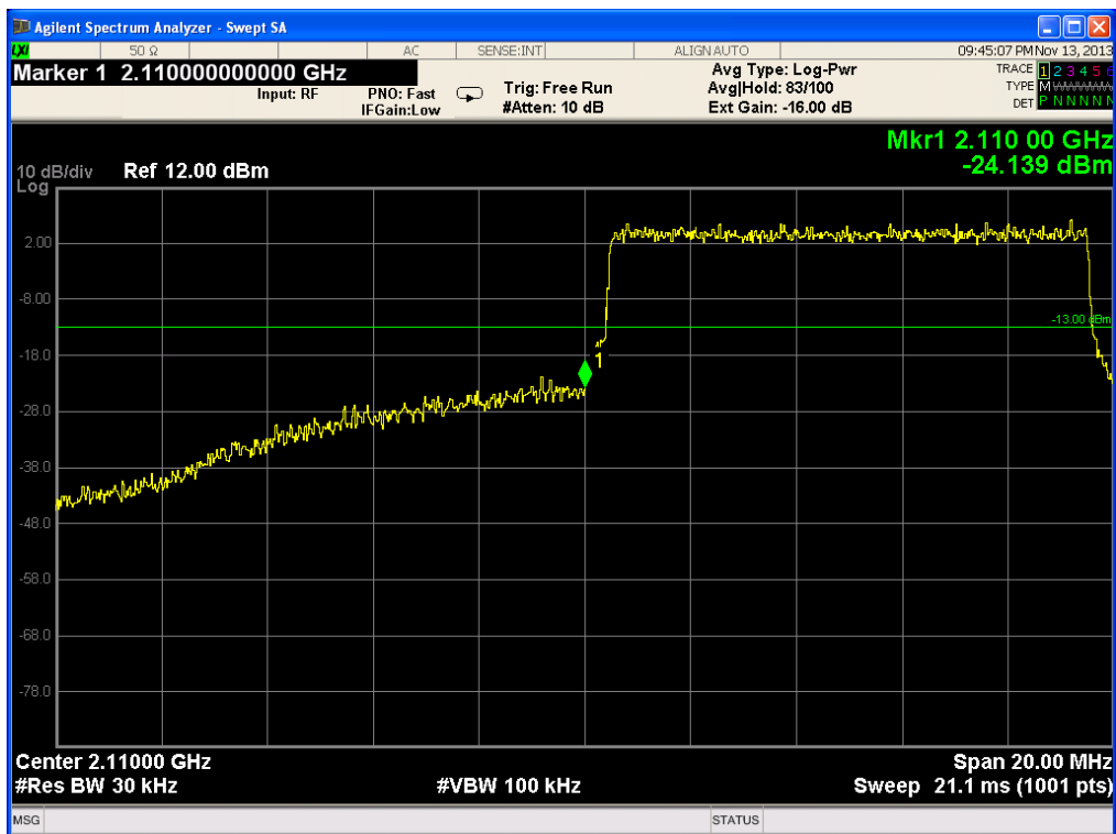
Figure 50.— 64QAM LOW
