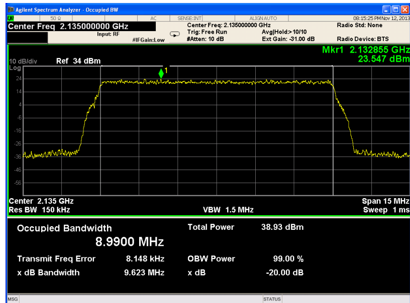
Figure 20.— 16QAM (MID CHANNEL) IN
