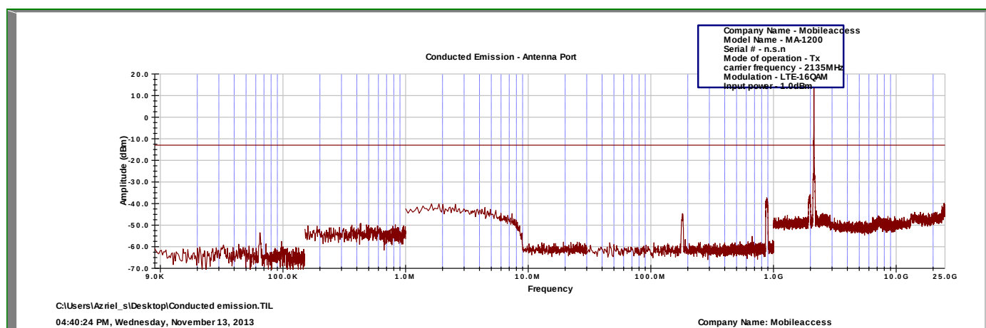
Figure 39.— 16QAM (Mid)
