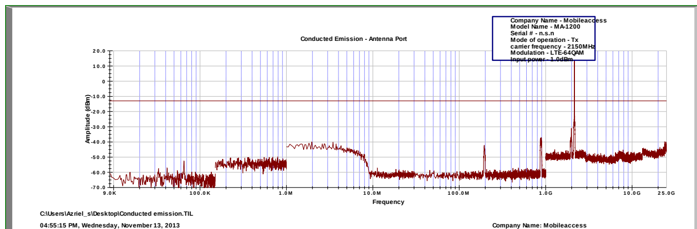
Figure 43.— 64QAM (High)
