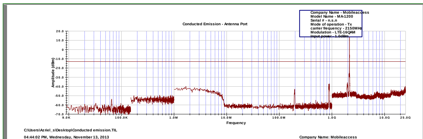
Figure 40.— 16QAM (High)
