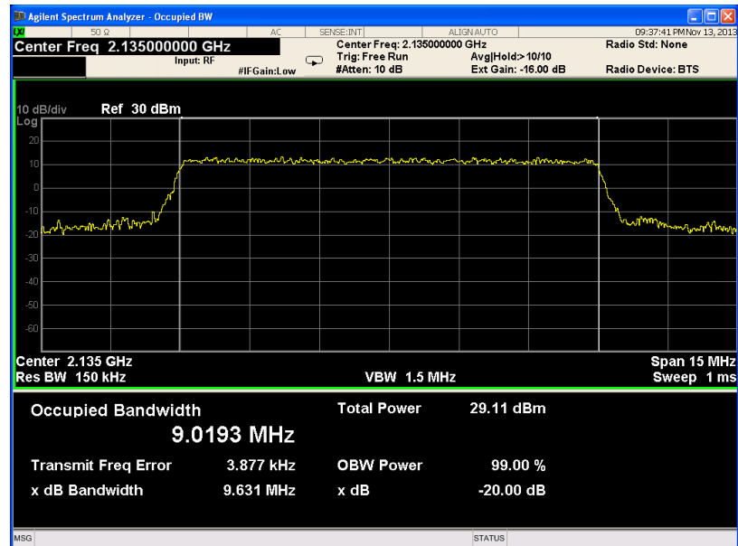
Figure 21.— 16QAM (MID CHANNEL) OUT
