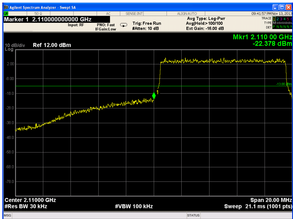
Figure 52.— QPSK LOW
