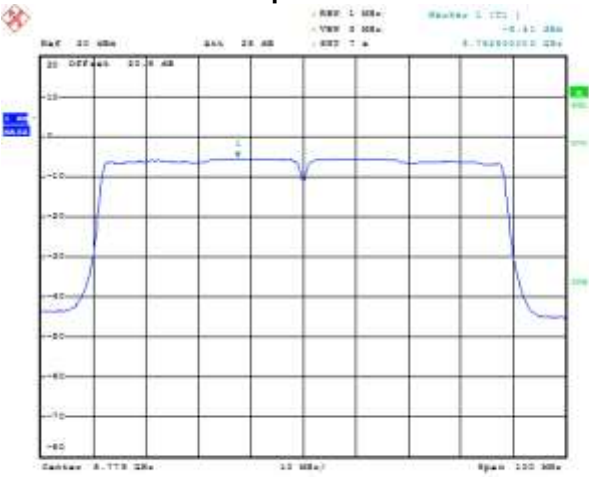
Figure 8-99: Peak Power Spectral Density SISO Primary, 802.11ac, Channel 155, MCS0 Mbps
