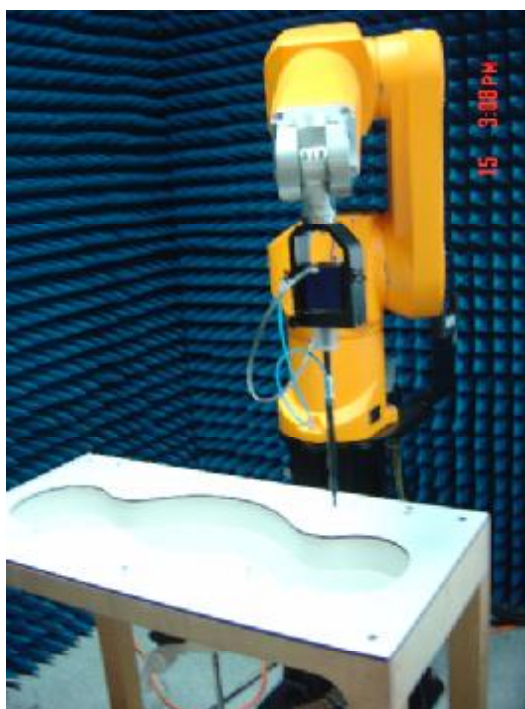
Fig.1 Photograph of the SAR measurement System
