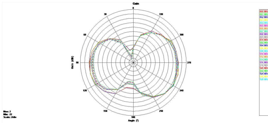
2D Radiation Pattern (Phi=90)
