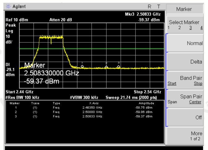
Right bandedge
