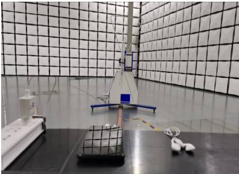
Radiated Emissions Test Setup (30-1000MHz)
