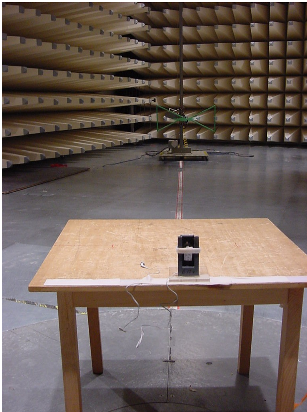
Photo 5 (Radiated Emissions): Headsets
