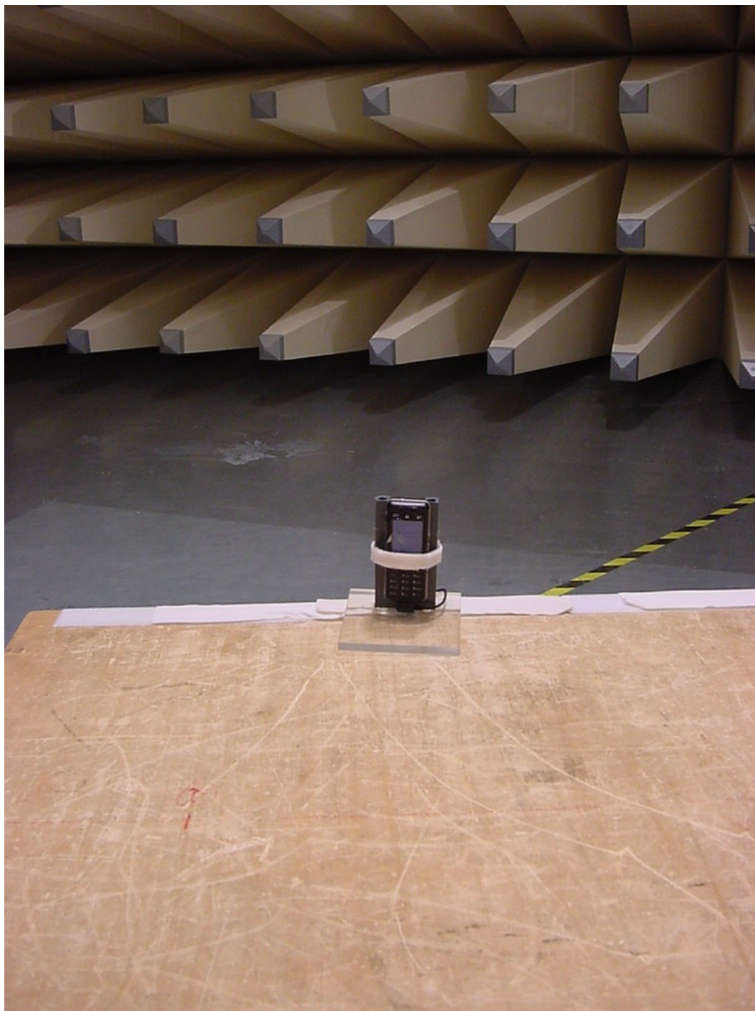
Photo 2 (Radiated Emissions): AC/DC Adapter (Charger )
