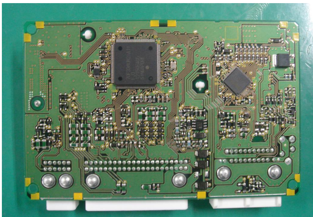
Figure 8.2 S79M0 PCB assy (bottom view)
