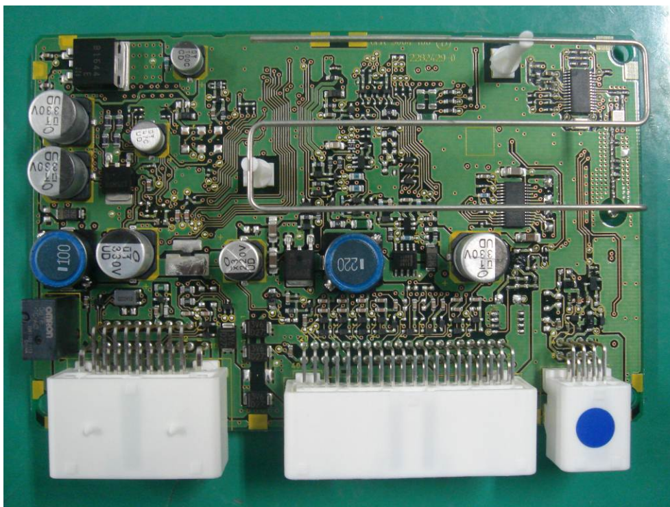
Figure 8.1 S79M0 PCB assy (top view)
