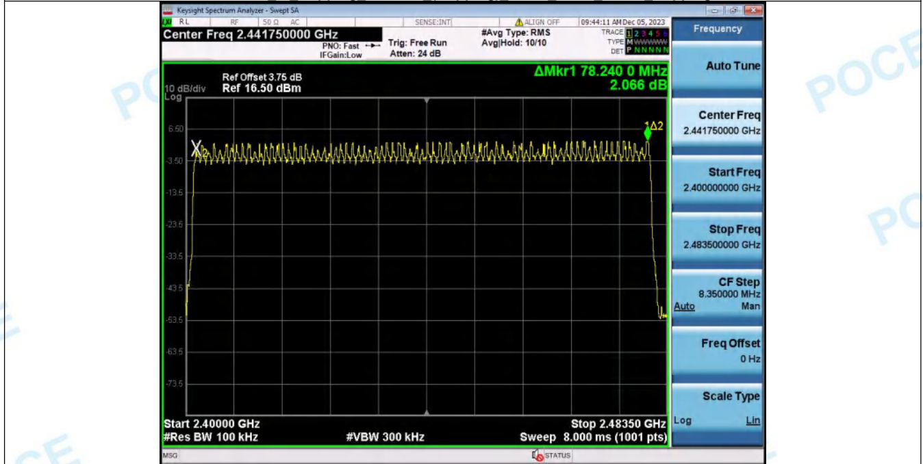
Number_of_Hopping_Channel_(Hopping)_NVNT_ANT1_2-DH5_Hopping
