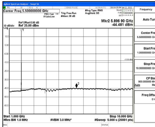
Band2-10MHz-16QAM-18900-1RB#0-Range5:10000~20000MHz
