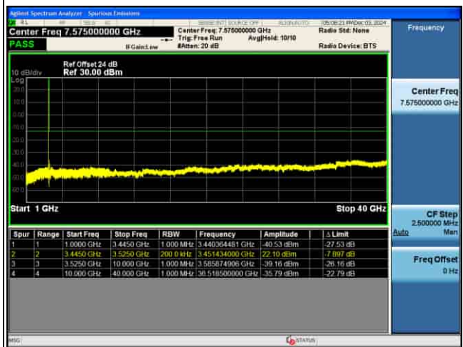
CSE_5G_n77(K)_30KHz_64QAM_70M CH633334_1RB@1_
