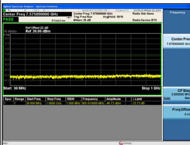
CSE_5G_n77(K)_30KHz_256QAM_15M CH633334_1RB@1_
