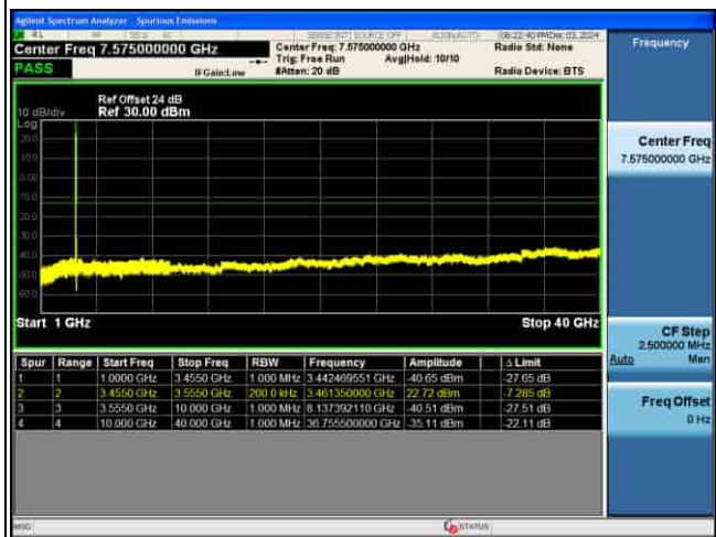
CSE_5G_n77(K)_30KHz_QPSK_100M CH633334_1RB@1_
