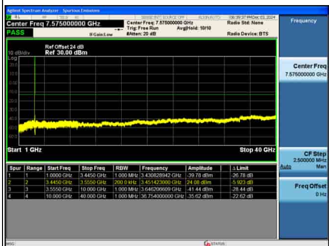
CSE_5G_n77(K)_30KHz_16QAM_10M CH630334_1RB@1_
