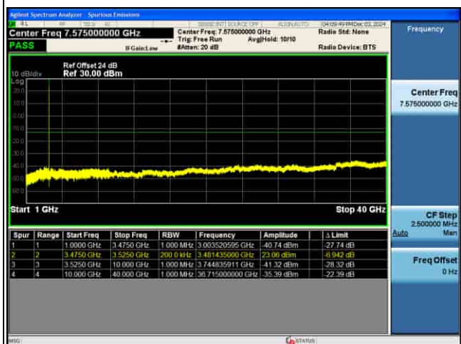
CSE_5G_n77(K)_30KHz_64QAM_40M CH635332_1RB@1_
