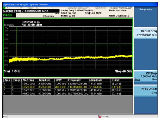
CSE_5G_n77(K)_30KHz_256QAM_100M CH633334_1RB@1_
