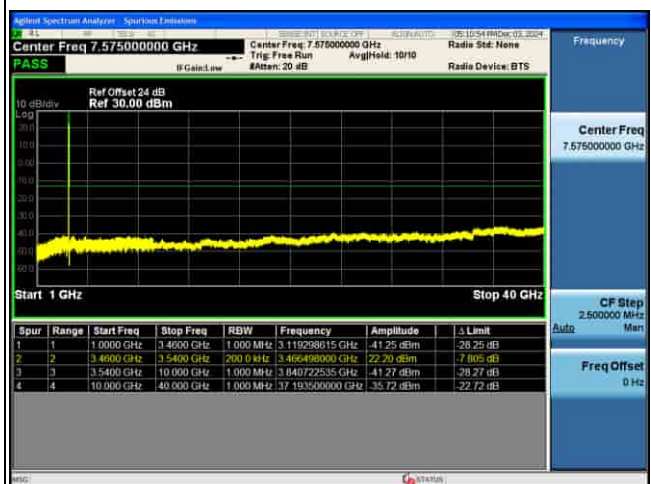
CSE_5G_n77(K)_30KHz_64QAM_70M CH634332_1RB@1_
