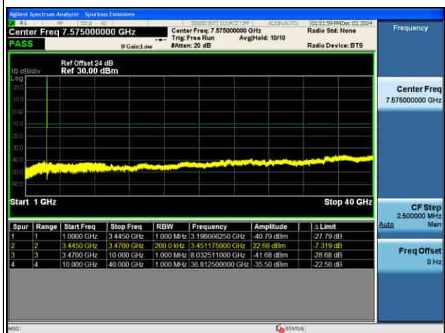
CSE_5G_n77(K)_30KHz_256QAM_15M CH633334_1RB@1_
