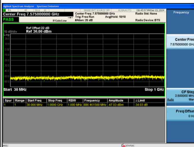
CSE_5G_n77(K)_30KHz_256QAM_100M CH633334_1RB@1_
