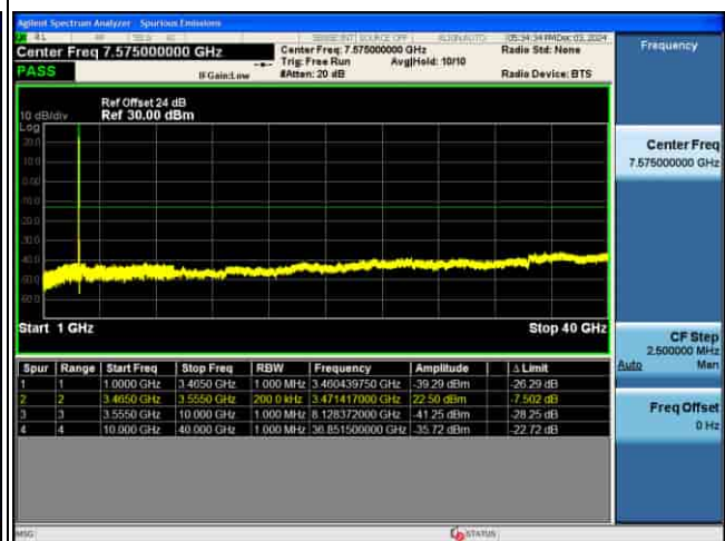
CSE_5G_n77(K)_30KHz_16QAM_90M CH633000_1RB@1_
