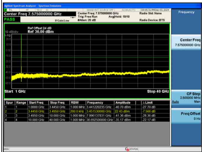
CSE_5G_n77(K)_30KHz_64QAM_40M CH633334_1RB@1_
