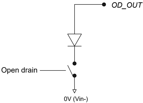
Figure 9 – SAT-IDP output block diagram
