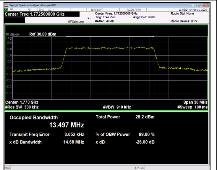
Band66-15MHz-16QAM-132597-75RB#0-PASS
