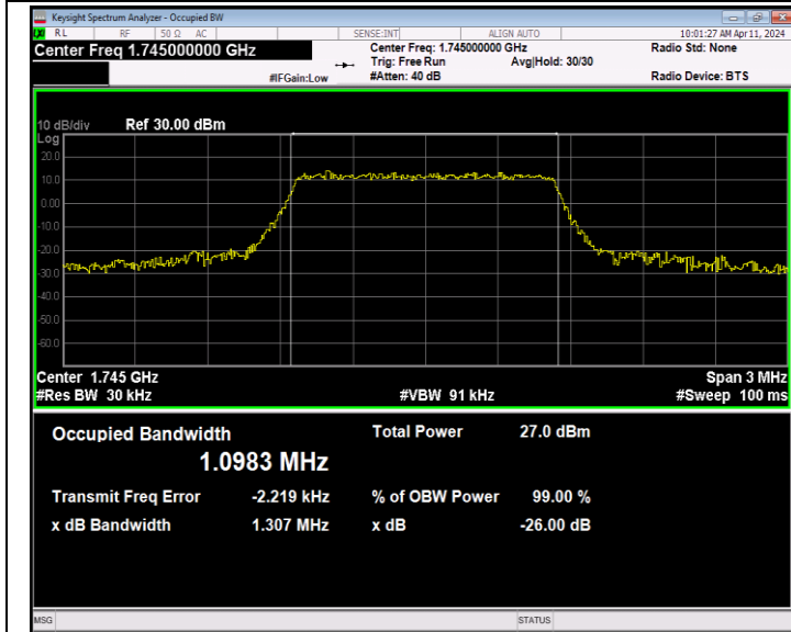
Band66-1.4MHz-16QAM-132322-6RB#0-PASS
