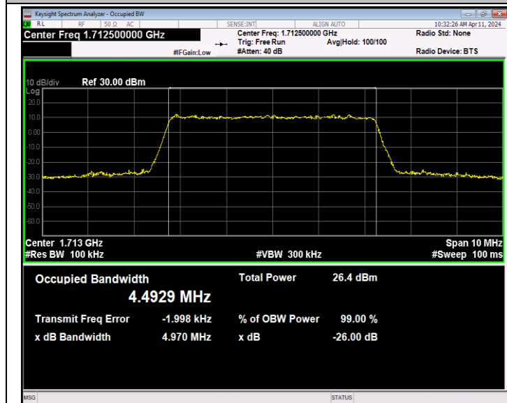
Band66-5MHz-64QAM-131997-25RB#0-PASS
