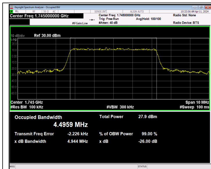
Band66-5MHz-16QAM-132322-25RB#0-PASS
