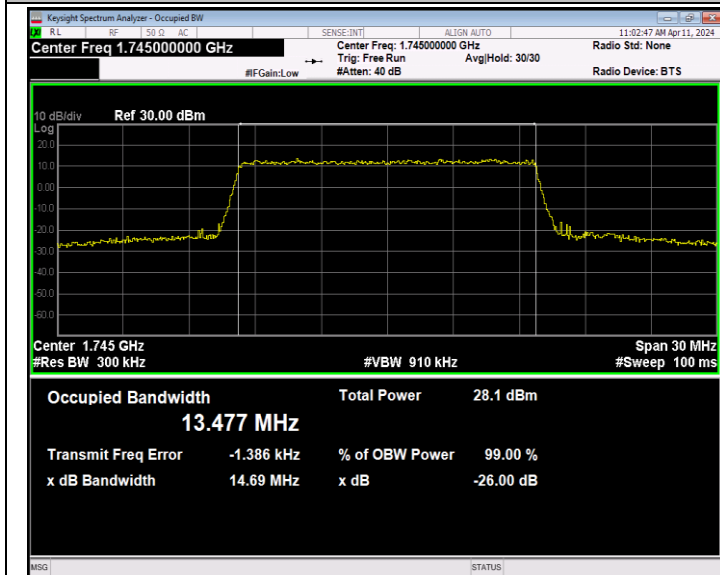
Band66-15MHz-16QAM-132322-75RB#0-PASS
