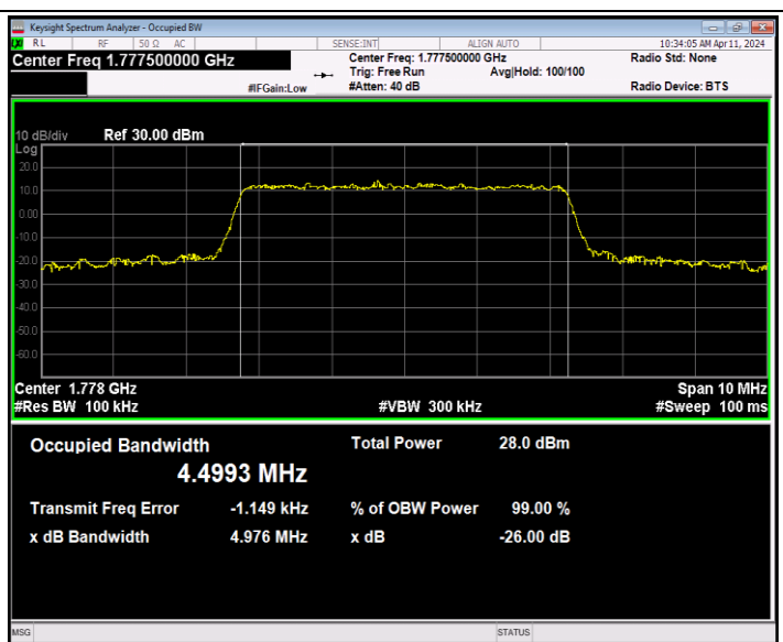
Band66-5MHz-16QAM-132647-25RB#0-PASS
