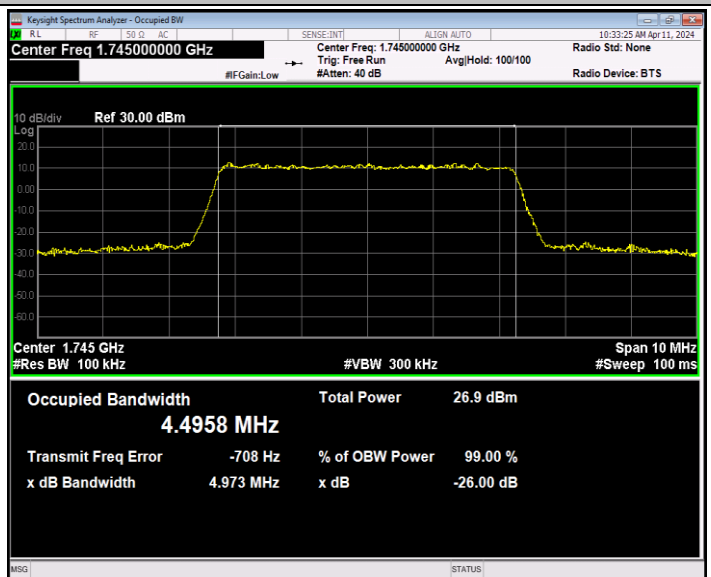
Band66-5MHz-64QAM-132322-25RB#0-PASS
