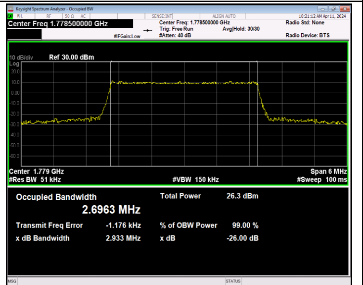
Band66-3MHz-64QAM-132657-15RB#0-PASS
