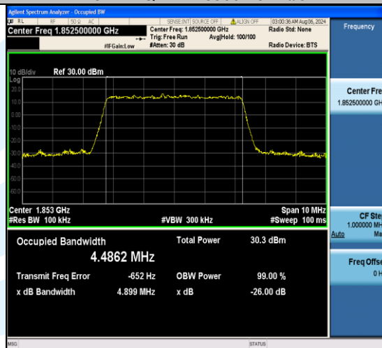
Band2-5MHz-16QAM-18625-25RB#0-PASS
