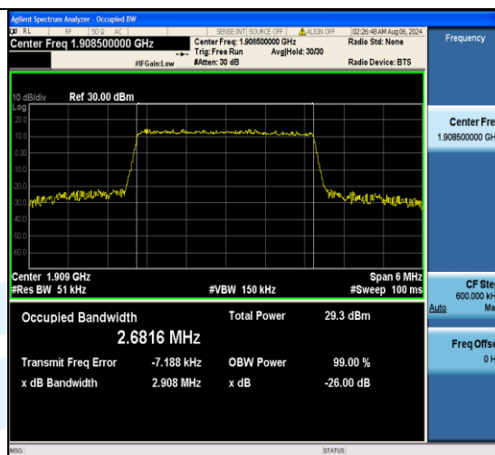
Band2-3MHz-16QAM-19185-15RB#0-PASS
