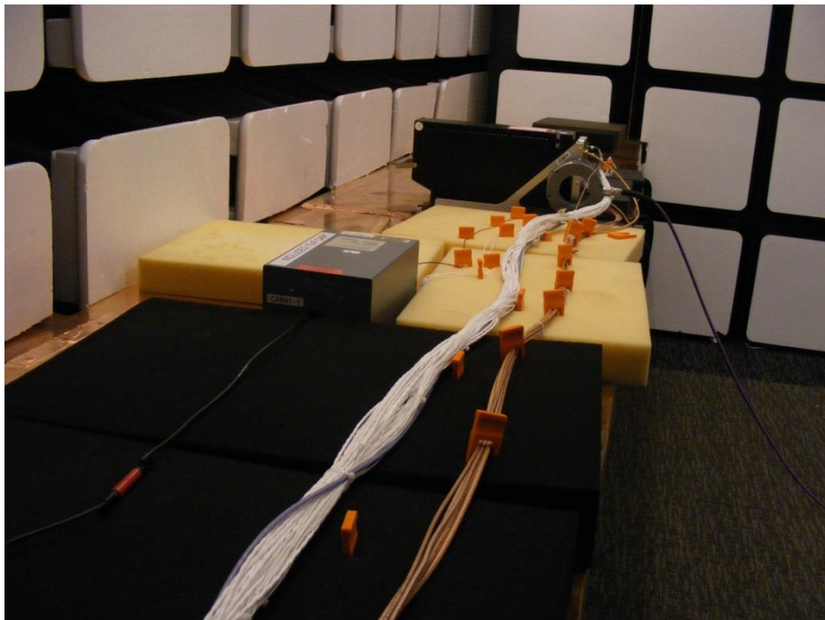
Figure 9 Cable Layout – Bulkhead Perspective
