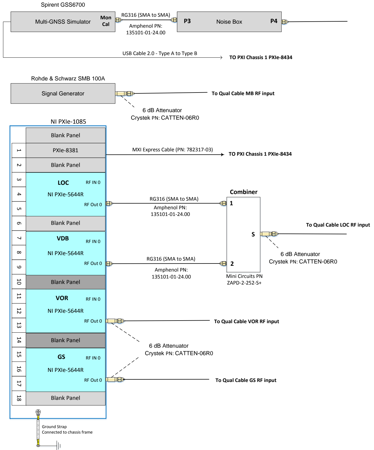
Figure 3 External generators for Flight Test Pallet (provided)
