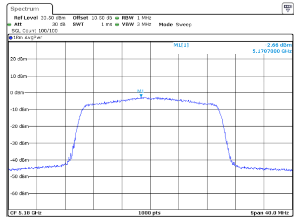
802.11ax20_5180MHz_RU_Full_Chain 2
