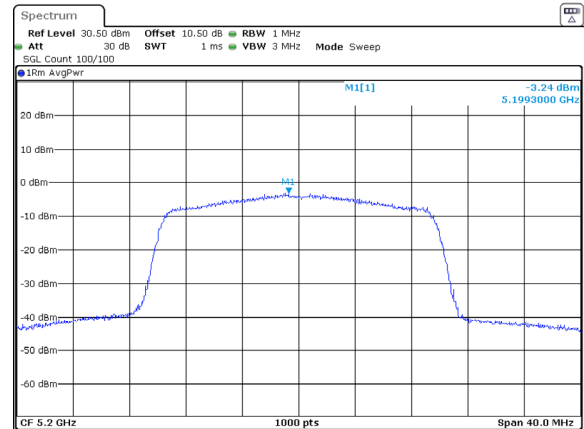
802.11ax20_5200MHz_RU_Full_Chain 1
