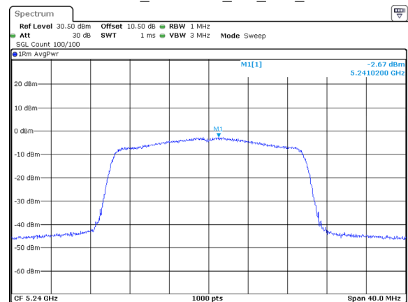
802.11ax20_5240MHz_RU_Full_Chain 2
