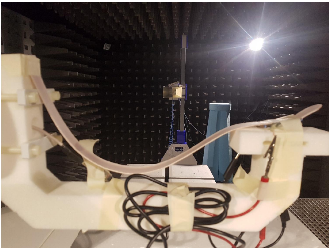
Test set up radiated emission 1GHz – 18GHz
