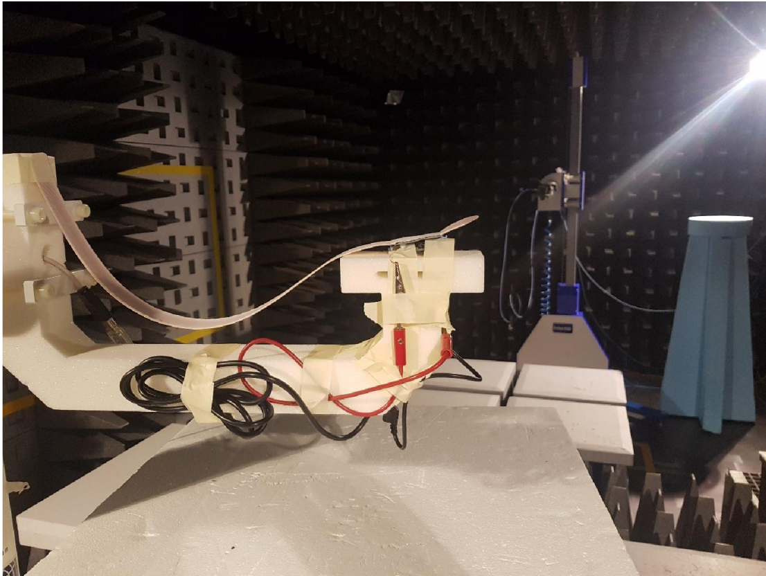
Test set up radiated emission 18GHz – 26GHz
