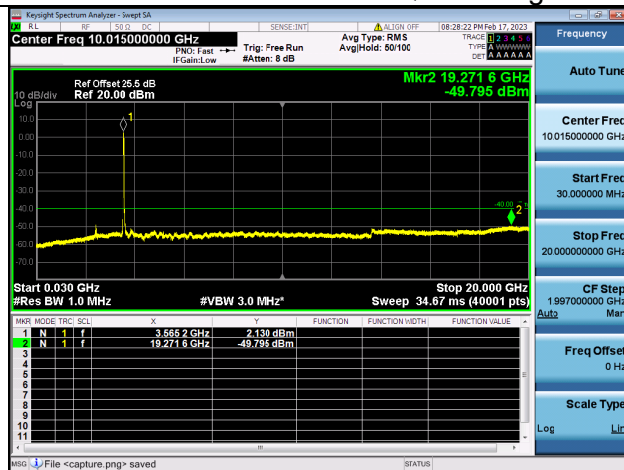
Band42C(3550~3600)-30M-20G / 20MHz+20MHz / 100RB+100RB/ QPSK / High CH
