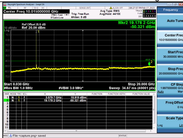
Band42C(3550~3600)-30M-20G / 20MHz+20MHz / 1RB+1RB/ QPSK / High CH
