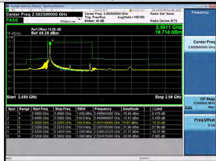
Band7-20MHz-16QAM-20850-27RB#0
