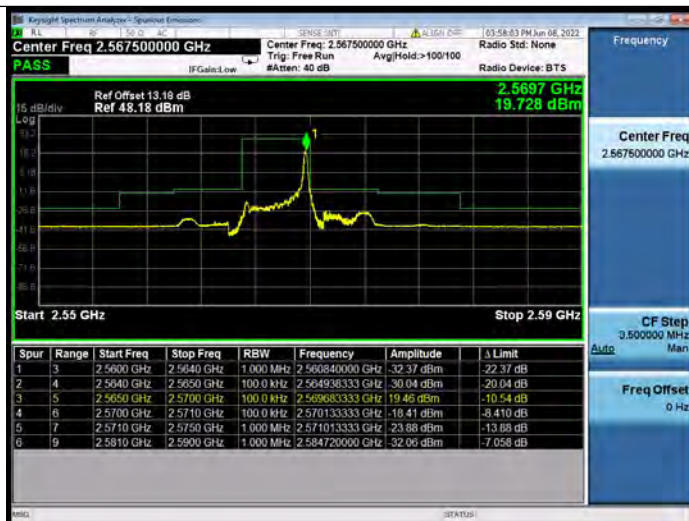
Band7-5MHz-16QAM-21425-25RB#0
