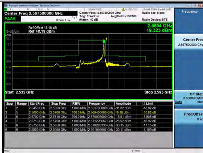
Band7-10MHz-16QAM-21400-27RB#23
