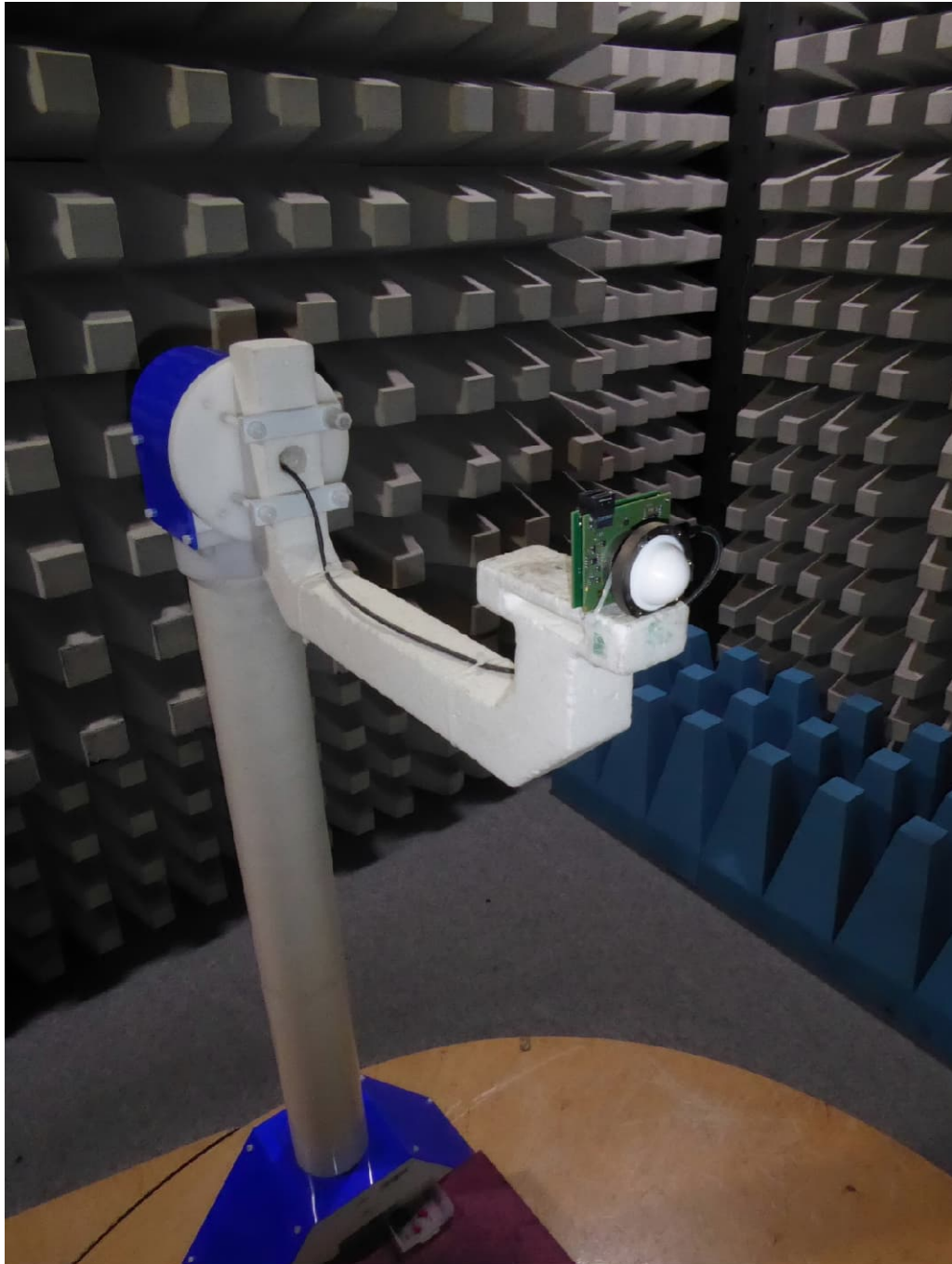
Test setup fully anechoic chamber (<40 GHz)
