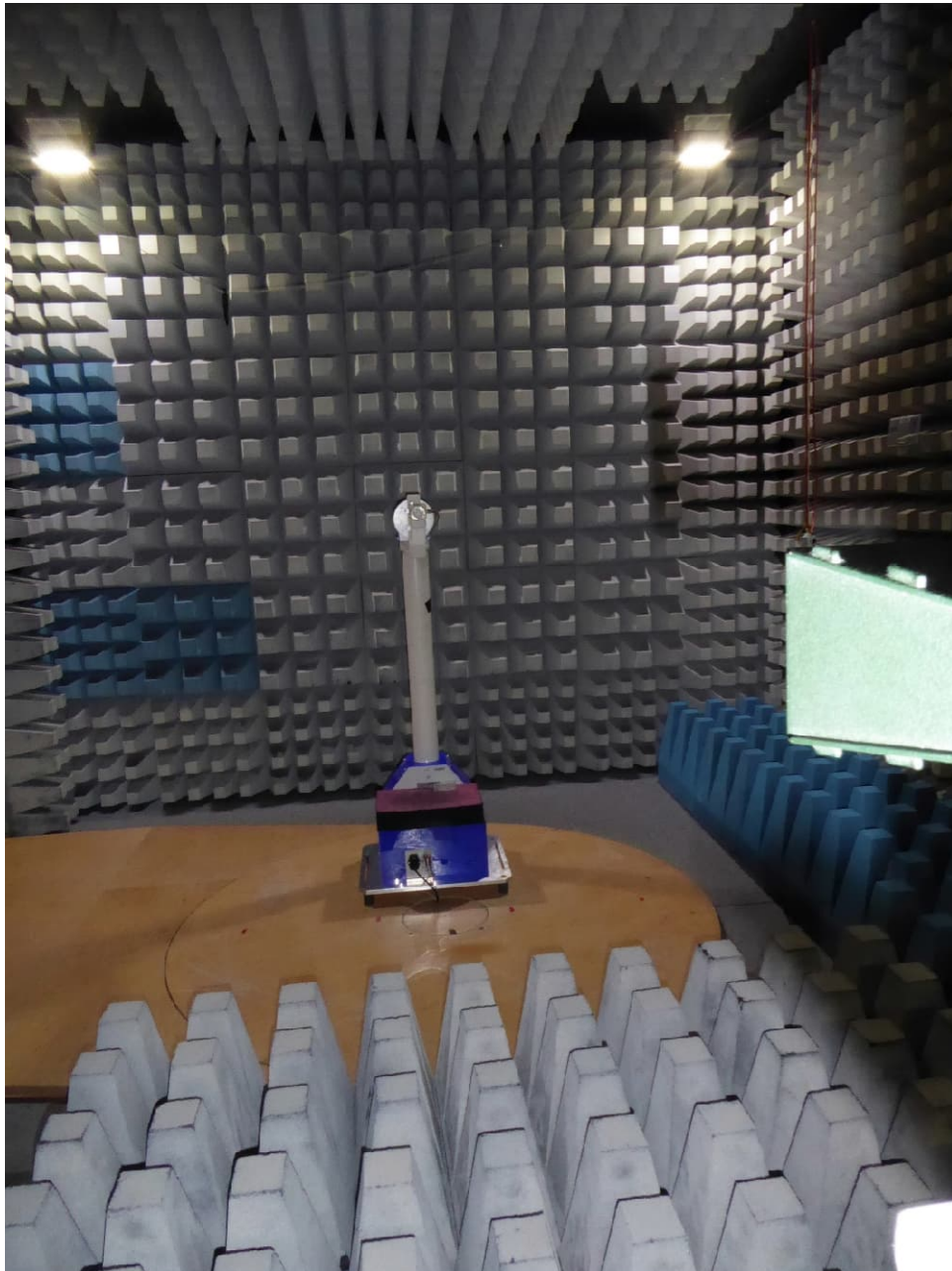
Test setup fully anechoic chamber (12 GHz to 26.5 GHz)
