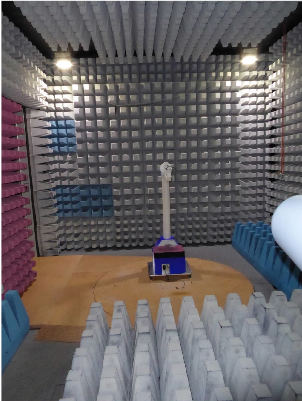
Test setup fully anechoic chamber (1 GHz to 12 GHz)
