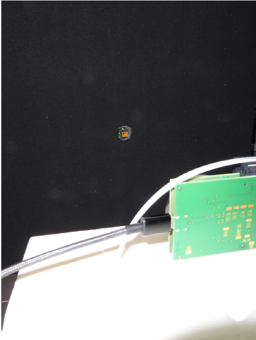
Test setup fully anechoic chamber with (>40 GHz)
