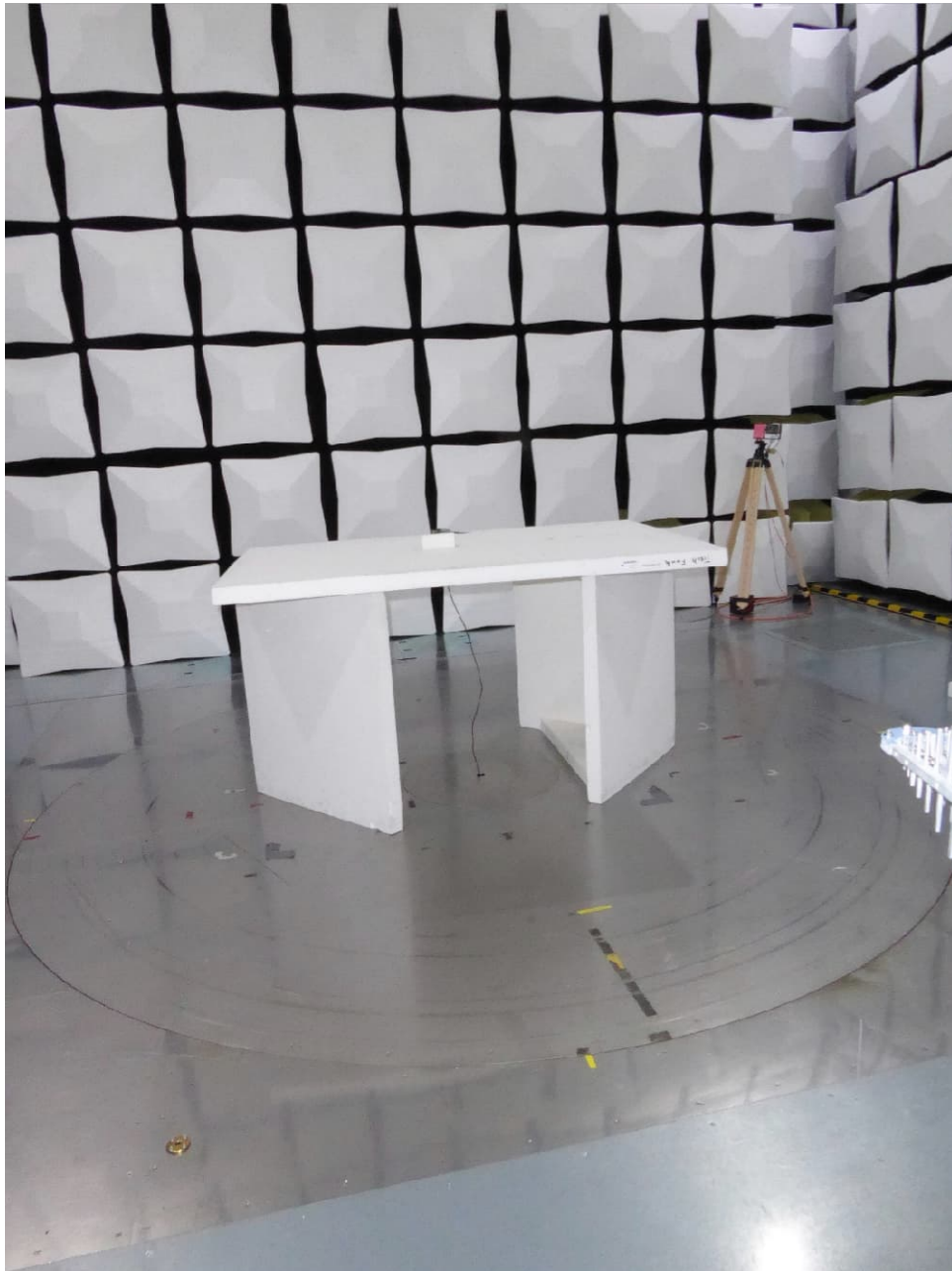
Test setup semi anechoic chamber (<1 GHz, position 1)
