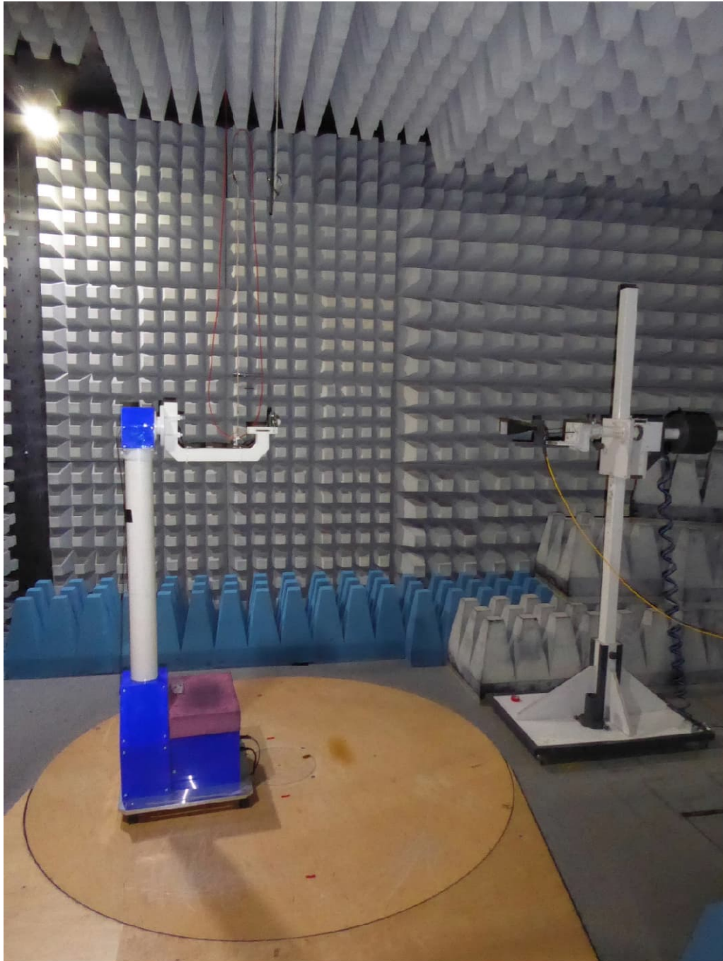
Test setup fully anechoic chamber (26.5 GHz to 40 GHz)
