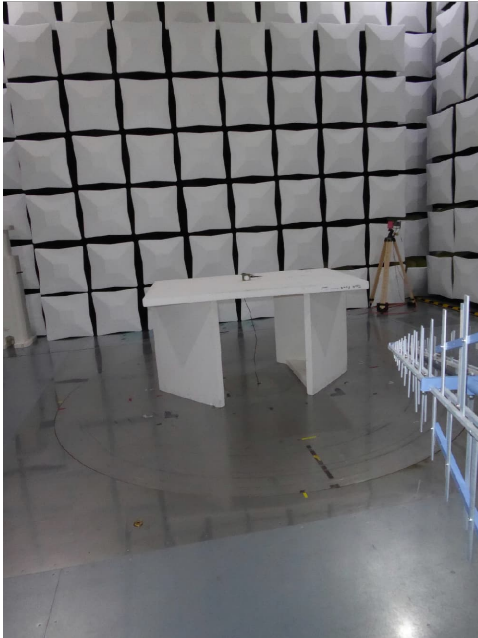
Test setup semi anechoic chamber (<1 GHz, position 2)
