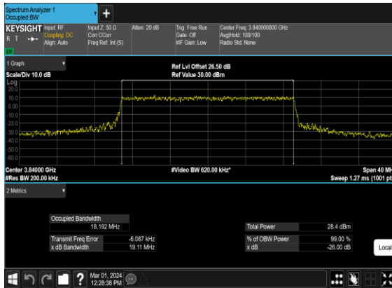
B13_N77(20M)_CP- OFDM_QPSK_Outer_Full_Mid_CH
