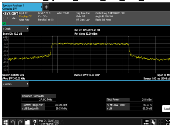
B13_N77(30M)_CP- OFDM_QPSK_Outer_Full_Mid_CH
