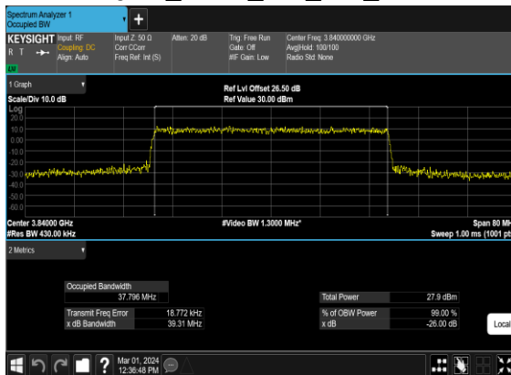
B13_N77(40M)_CP-OFDM_64 QAM_Outer_Full_Mid_CH
