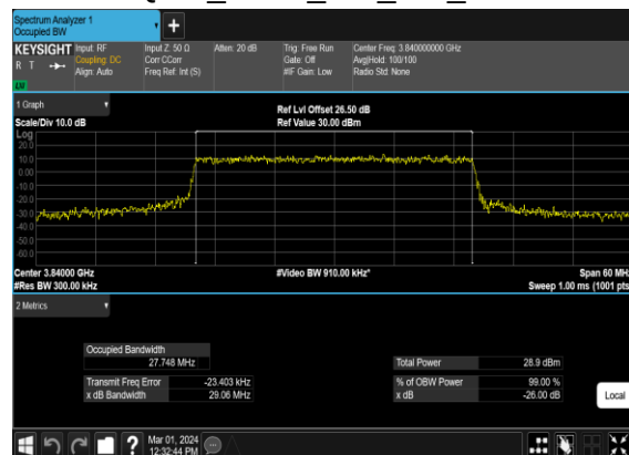
B13_N77(30M)_CP-OFDM_16 QAM_Outer_Full_Mid_CH
