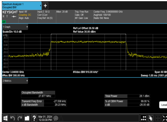
B13_N77(30M)_CP-OFDM_64 QAM_Outer_Full_Mid_CH
