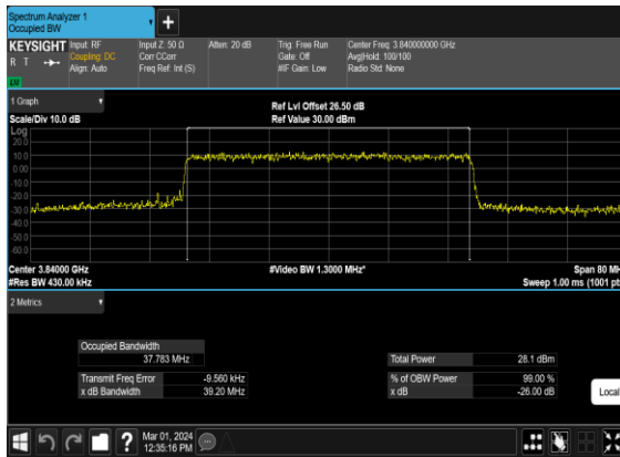
B13_N77(40M)_CP- OFDM_QPSK_Outer_Full_Mid_CH
