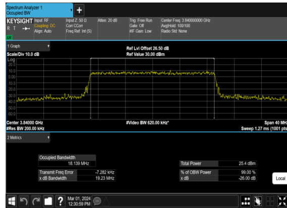
B13_N77(20M)_CP-OFDM_256 QAM_Outer_Full_Mid_CH
