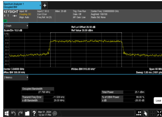
B13_N77(30M)_CP-OFDM_256 QAM_Outer_Full_Mid_CH
