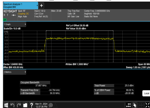
B13_N77(40M)_CP-OFDM_256 QAM_Outer_Full_Mid_CH
