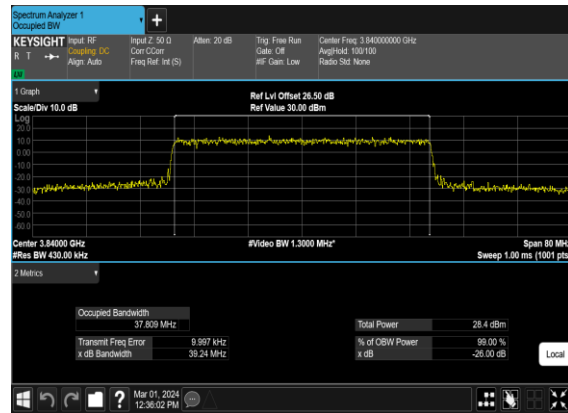
B13_N77(40M)_CP-OFDM_16 QAM_Outer_Full_Mid_CH
