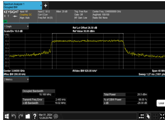
B13_N77(20M)_CP-OFDM_16 QAM_Outer_Full_Mid_CH
