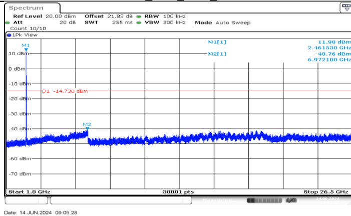
11B-CDD_Ant4_2462_1000-26500
