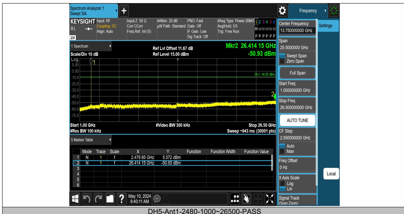
DH5-Ant1-2480-1000~26500-PASS
