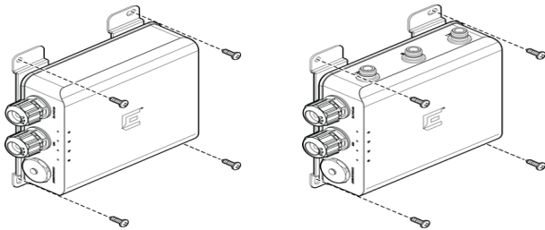
Figure 4 AP3917i/AP3917e Wall Mount "H" Bracket
