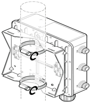
Figure 6 AP with Mounting Bracket—Vertical Pole
