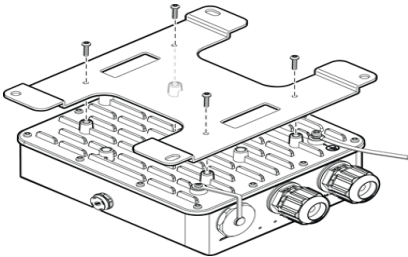
Figure 3 Attaching the "H" Bracket to the AP
