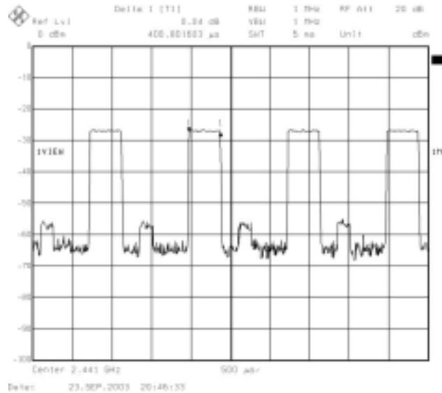
DH1 2441MHz
