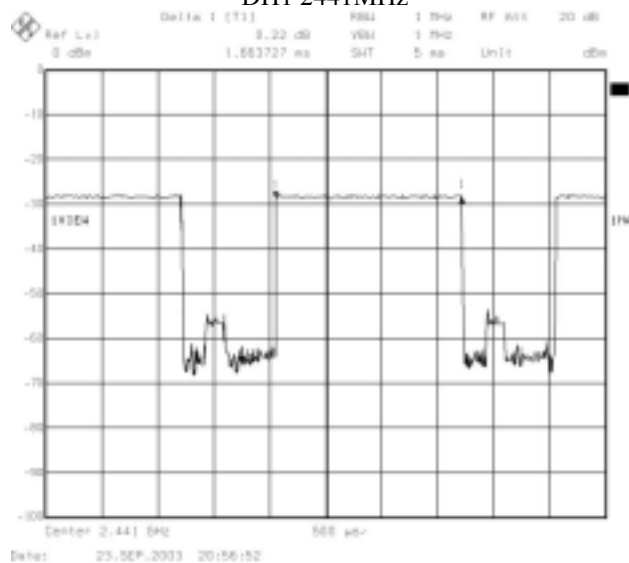
DH3 2441MHz
