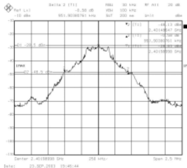
Channel Low
