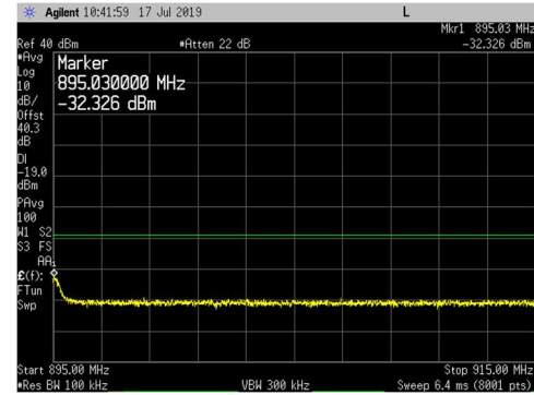
QPSK_Top Channel_ 895 to 915MHz
