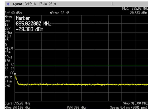
16QAM_ Top Channel_ 895 to 915MHz
