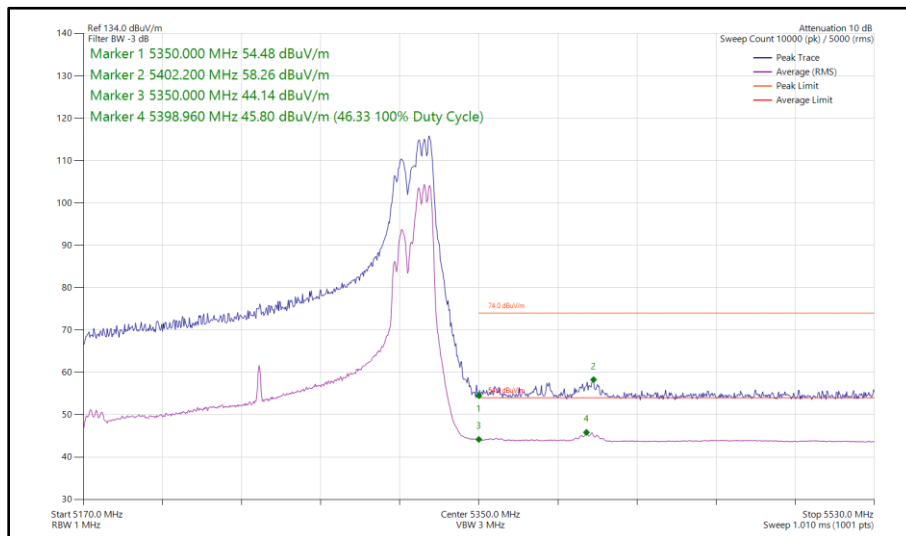
Figure 220 - 802.11ax HE160, RU 106-60S, SDM, Core 0 - Core 1 - 5250 MHz Band Edge Frequency 5350 MHz
