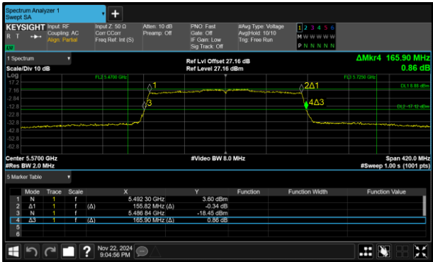
Figure 241 - 802.11ax HE160 SU Maximum 26 dB EBW
