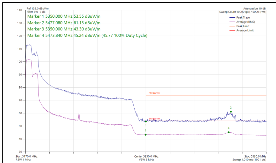
Figure 193 - 802.11ax HE160, RU 106-53P, SISO, Core 0 - 5250 MHz Band Edge Frequency 5350 MHz
