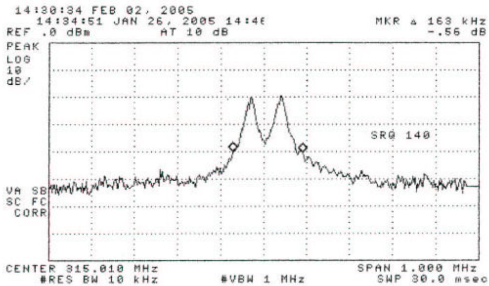
Figure 6.3. Measured bandwidth of the DUT (pulsed emission).
