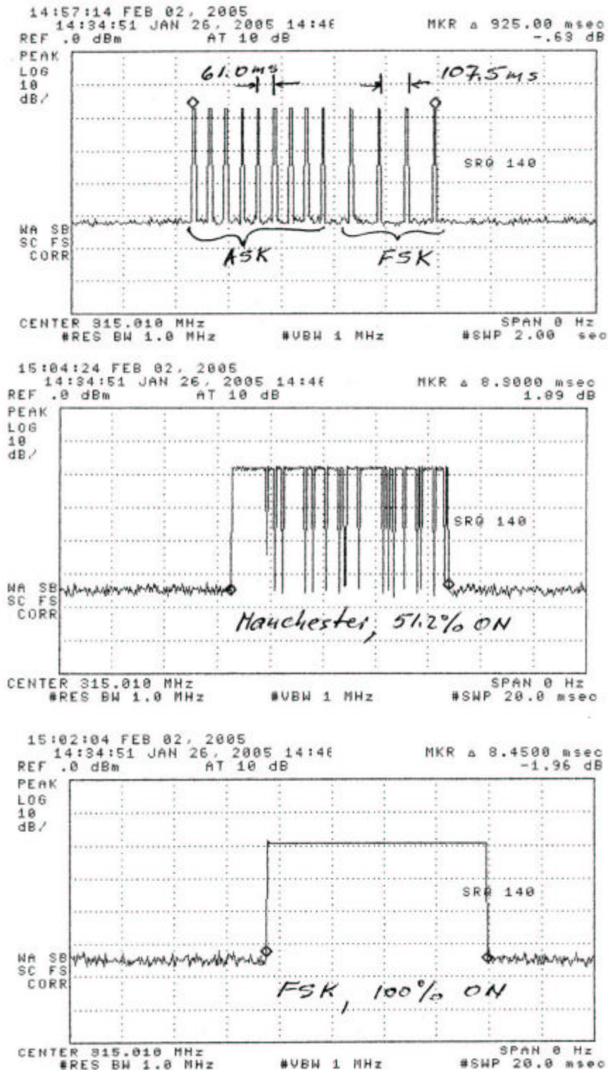
Figure 6.1. Transmissions modulation characteristics: (top) complete transmission, (center) expanded ASK, (bottom) expanded FSK.
